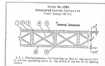
one hour floor assembly
