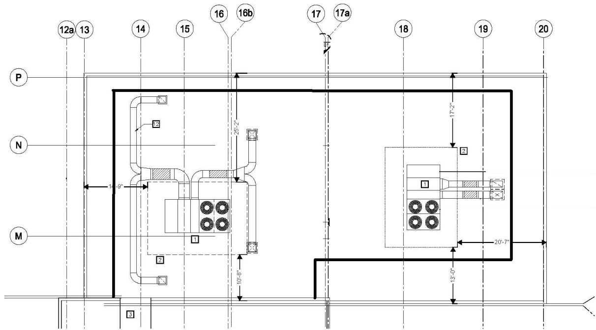
2 PART ROOF PLAN SCALE: 1/8" = 1'-0"
