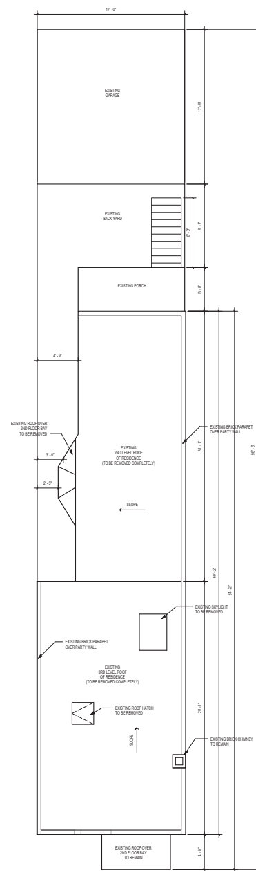
1 EXISTING SITE & ROOF PLAN 1/4" = 1'-0"
