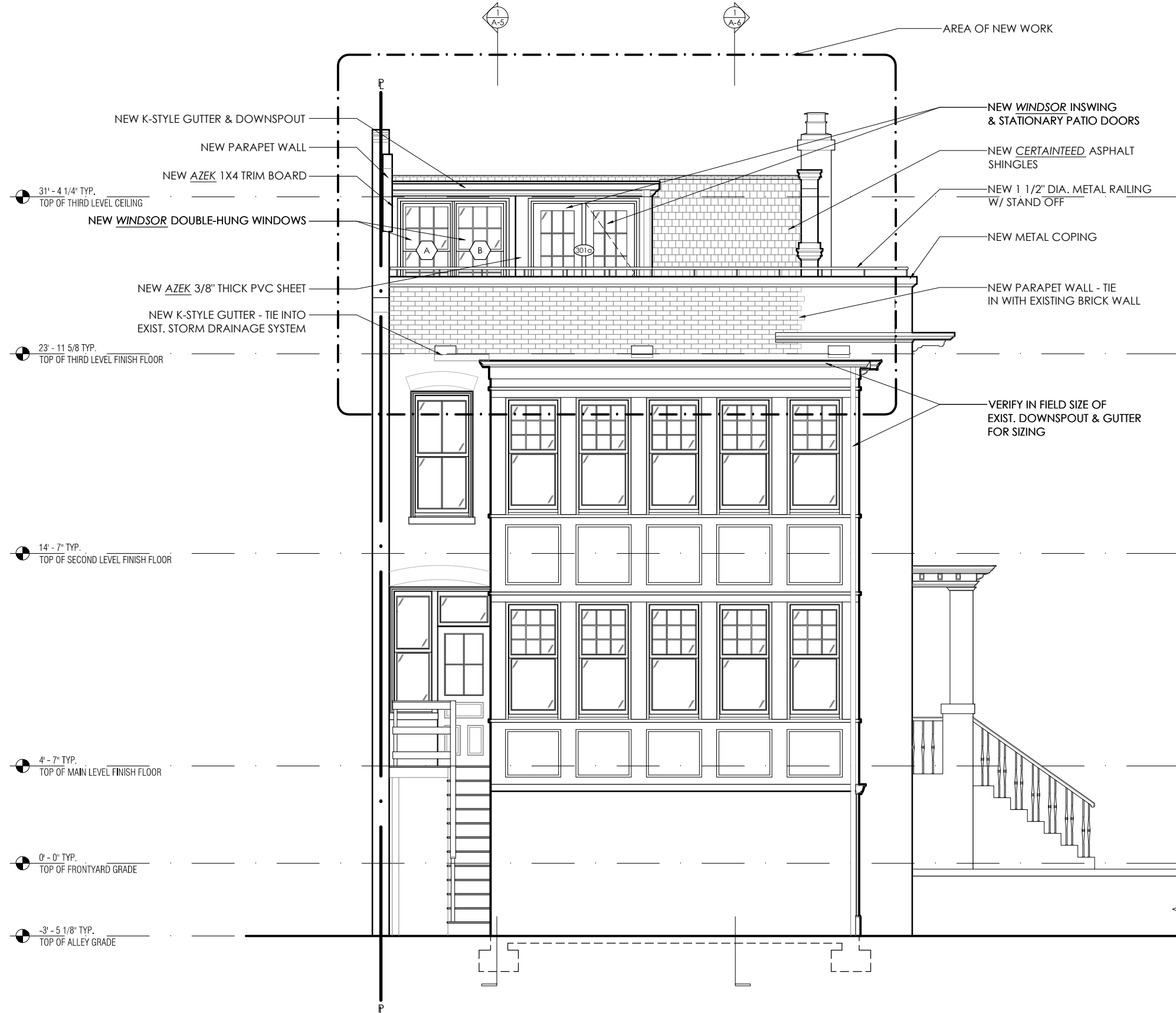
1 NORTH ELEVATION SCALE: 3/16" = 1'-0"
