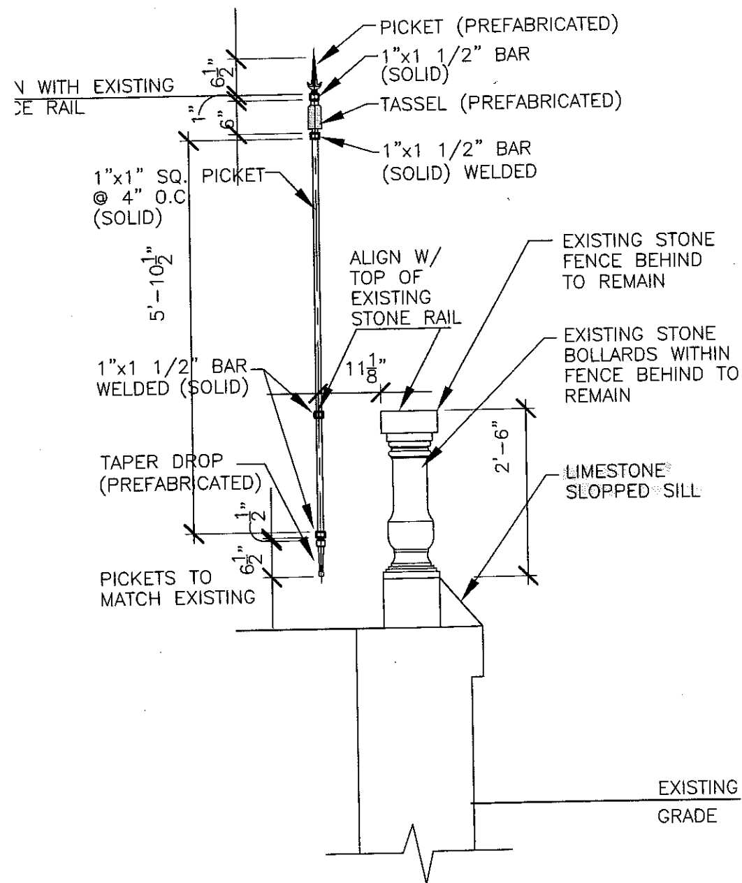
01 PICKET SECTION SCALE: 1/2"=1'-0"
