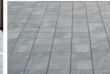
2" STONE PAVING on 1" sand setting bed and 4" concrete base over 4" of aggregate
