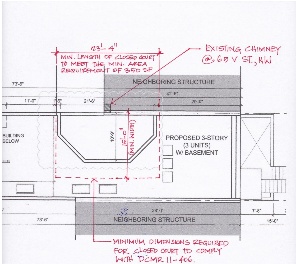
Diagram No. 1 – Partial Proposed Site Plan (Sheet A1.01): Dimensional and Area Requirements indicating non-compliance of the Court (Closed)
