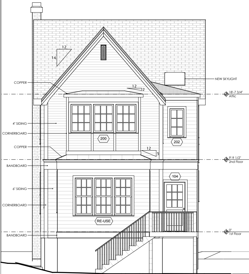
1 Rear Elevation 1/8" = 1'-0"
