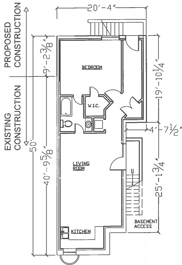
PROPOSED BASEMENT PLAN
