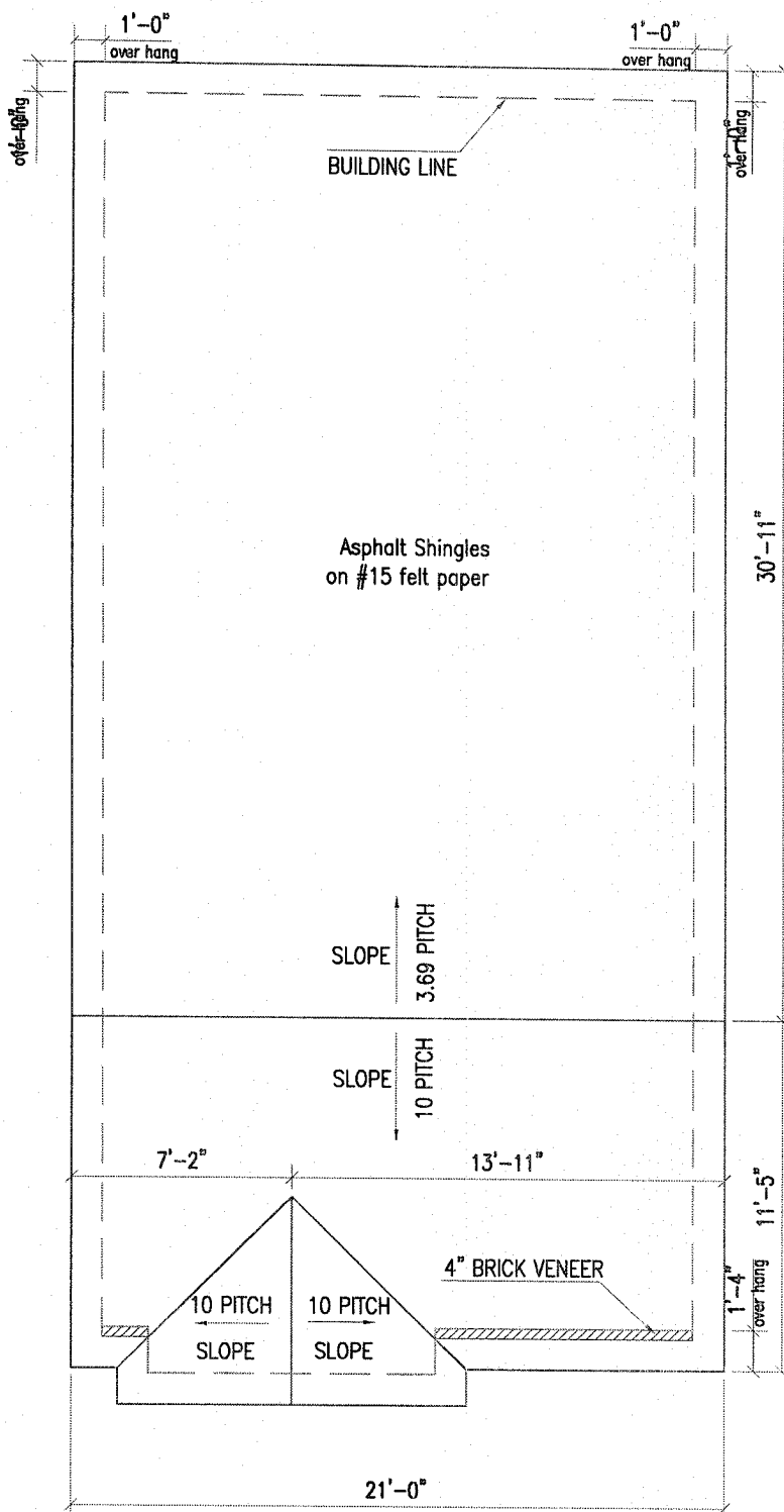
ROOF PLAN 4275 6TH ST SE
