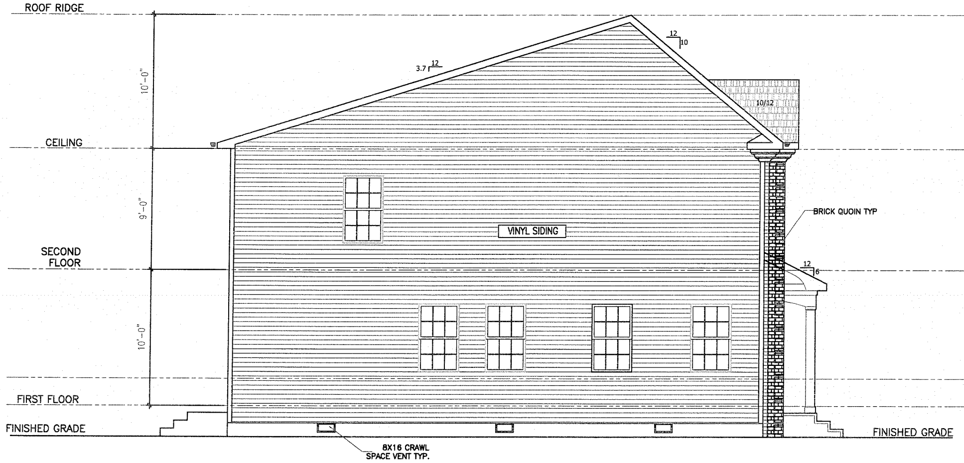
LEFT ELEVATION 4275 6TH ST SE
