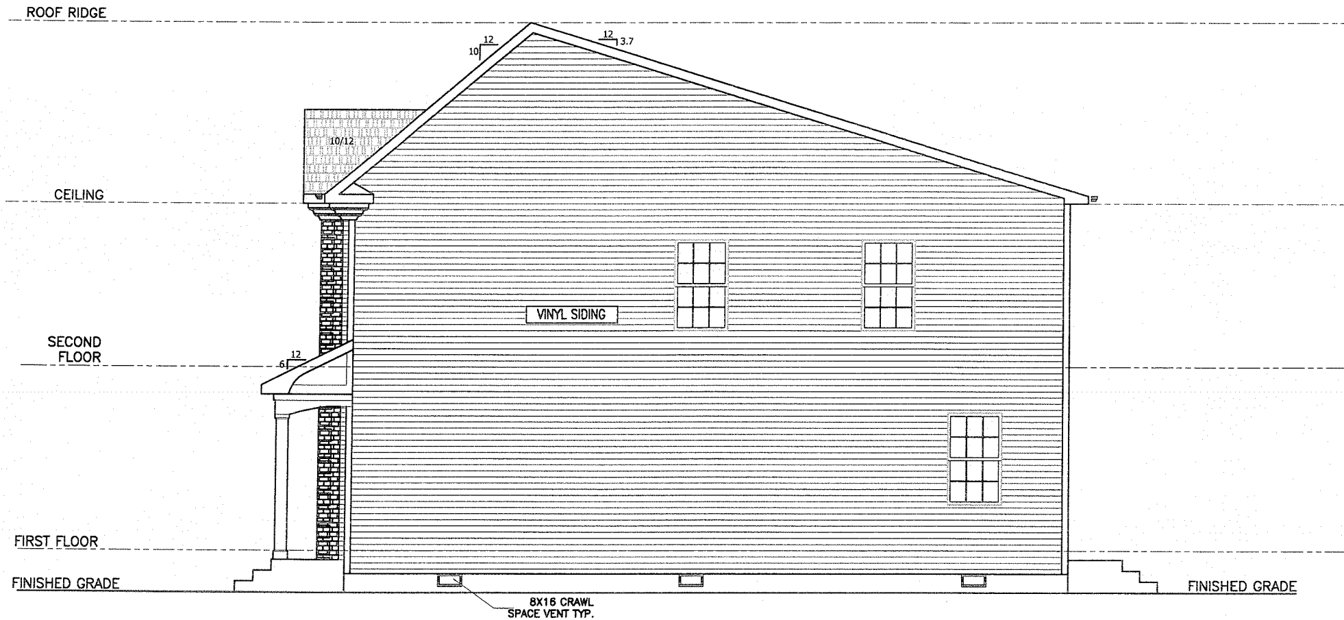
RIGHT ELEVATION 4275 6TH ST SE
