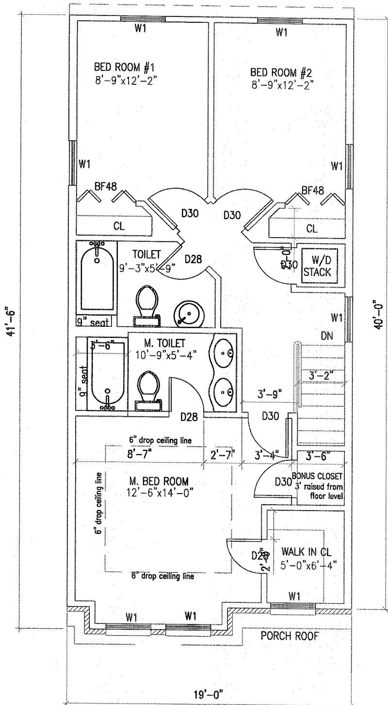
SECOND FLOOR PLAN 4275 6TH ST SE
