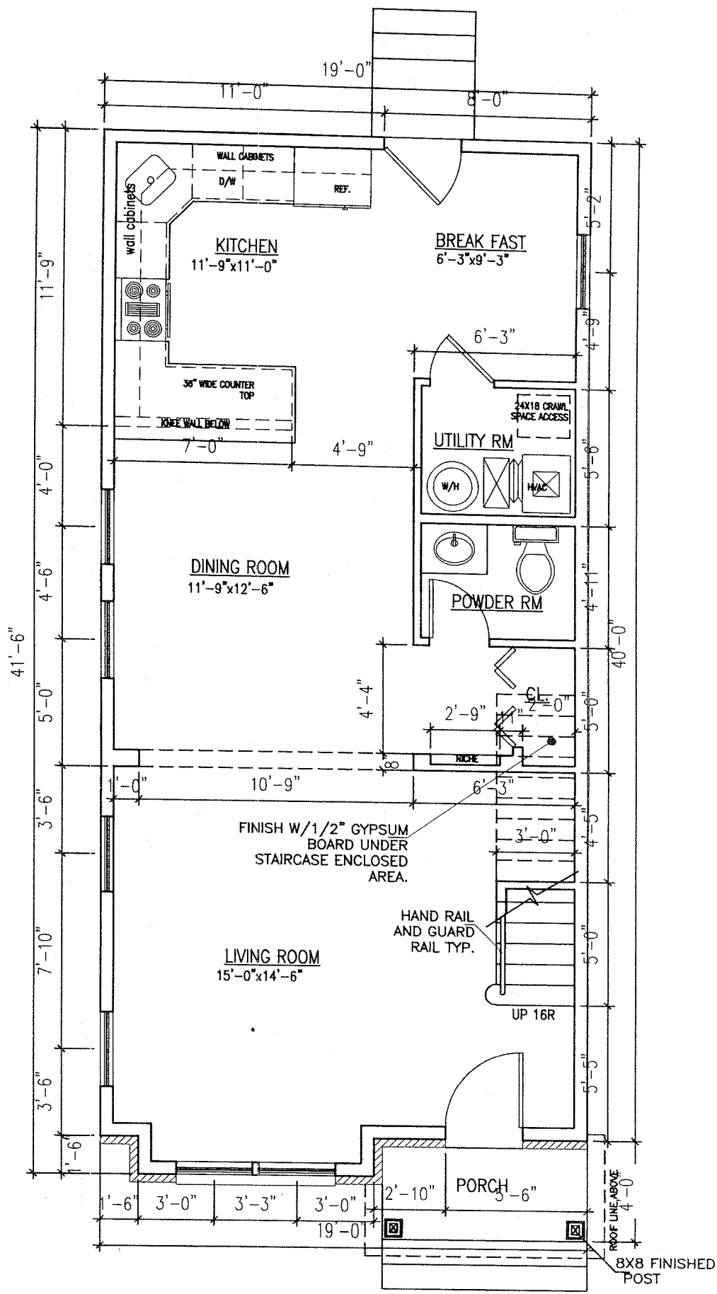
FIRST FLOOR PLAN 4926 FOOTE ST, NE
