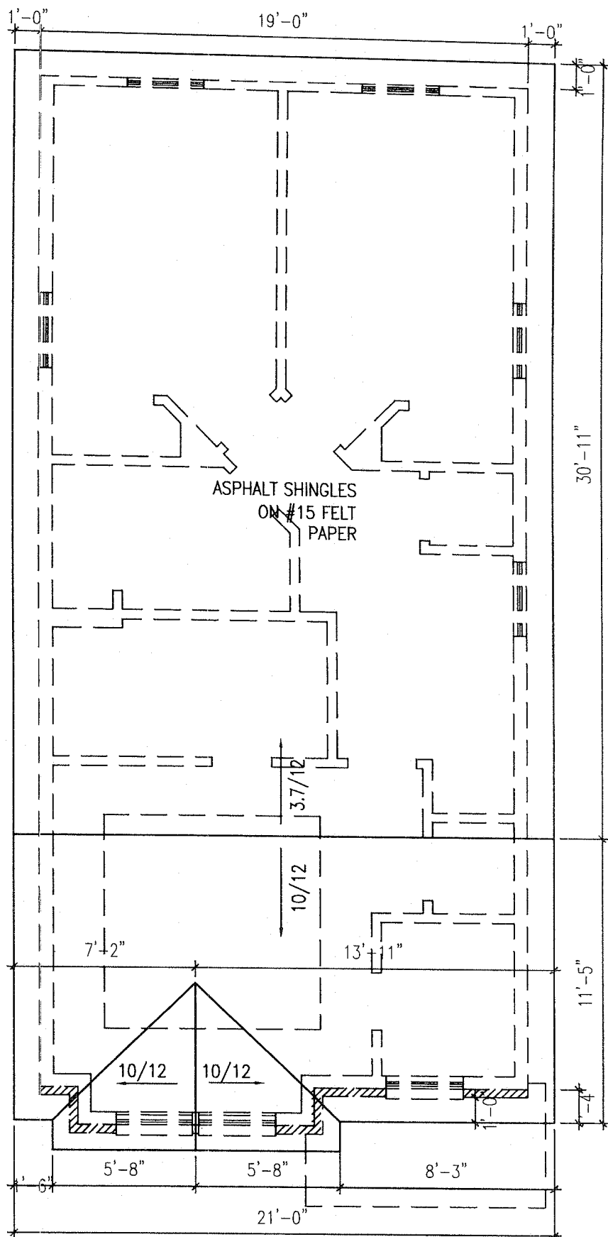
ROOF PLAN 4926 FOOTE ST, NE
