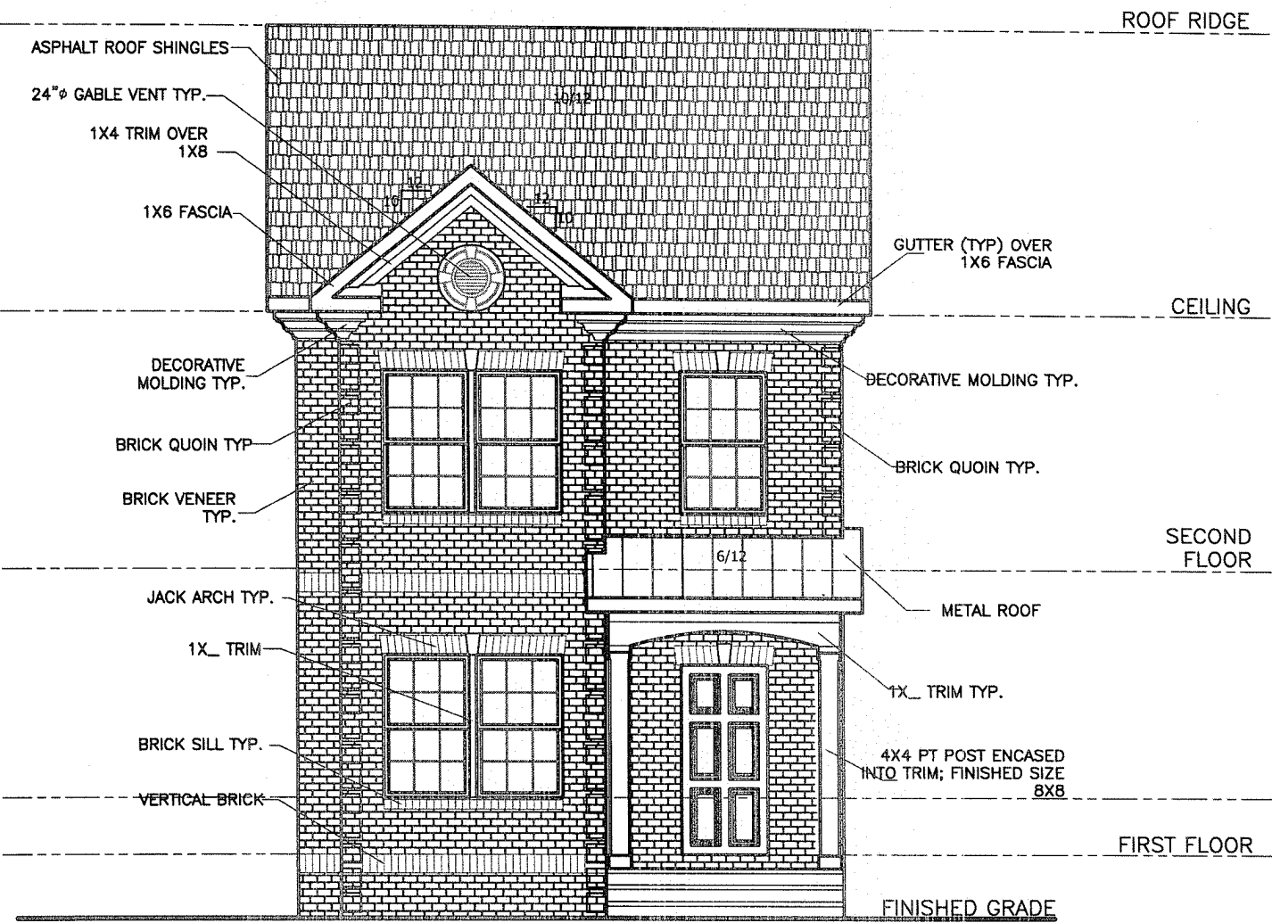
FRONT ELEVATION 6002 CLAY ST NE
