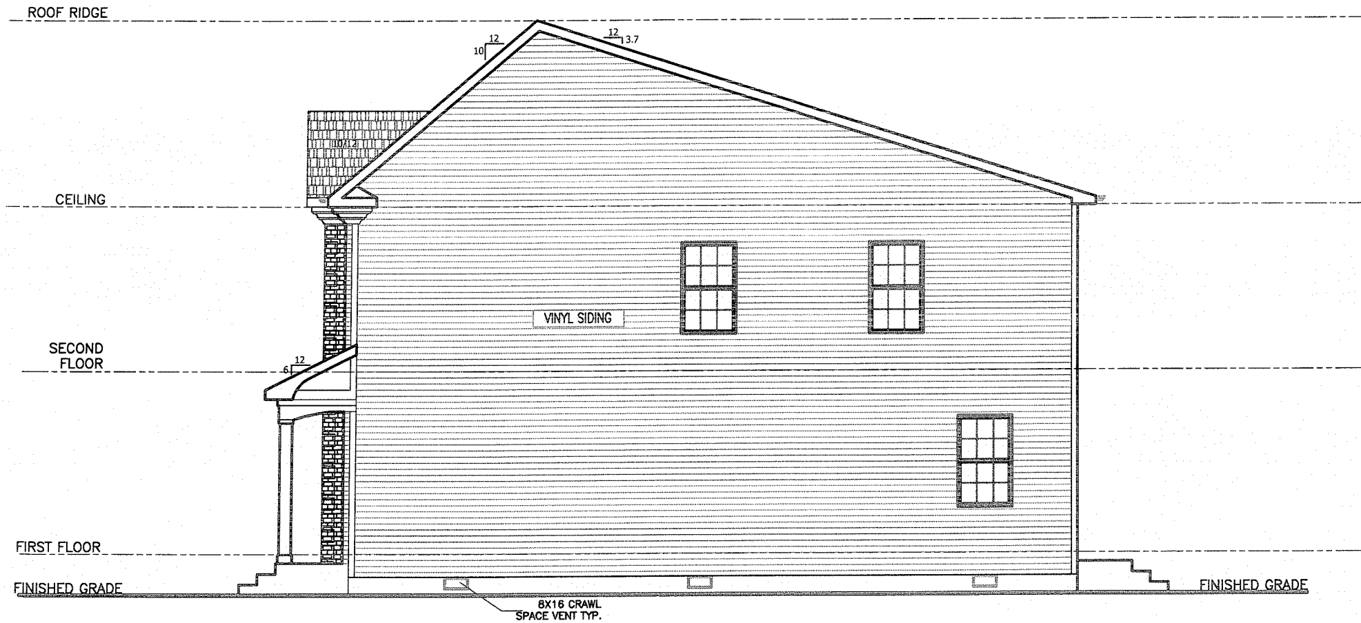
RIGHT ELEVATION 6002 CLAY ST NE
