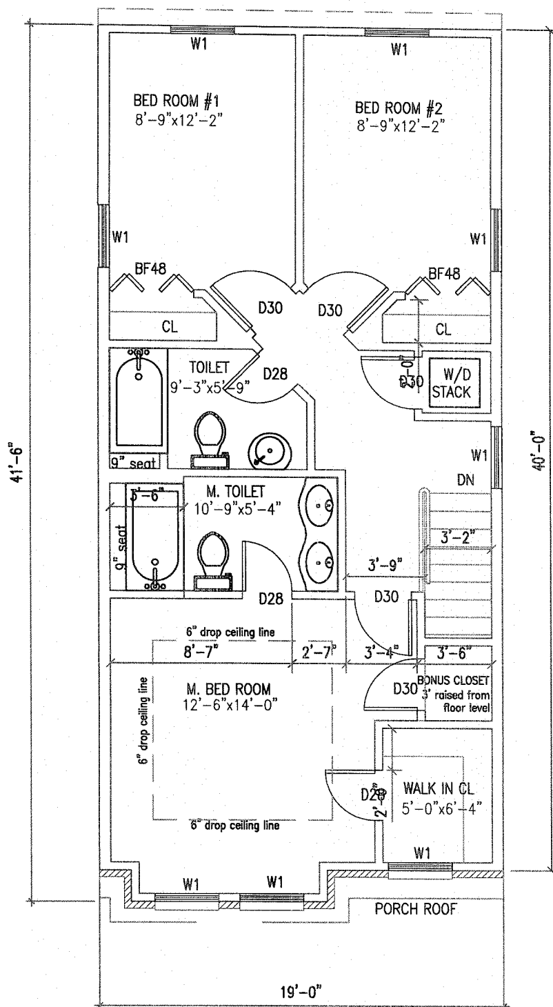
SECOND FLOOR PLAN 6002 CLAY ST NE
