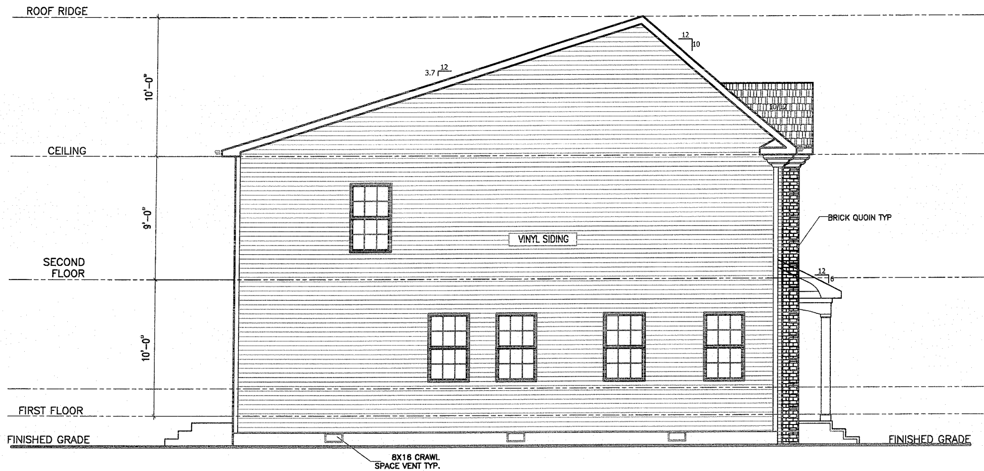
LEFT ELEVATION 6002 CLAY ST NE
