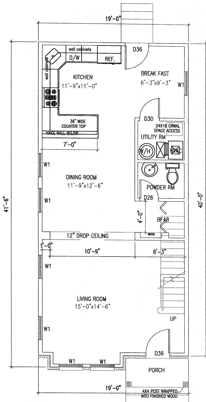
FIRST FLOOR PLAN 6002 CLAY ST NE
