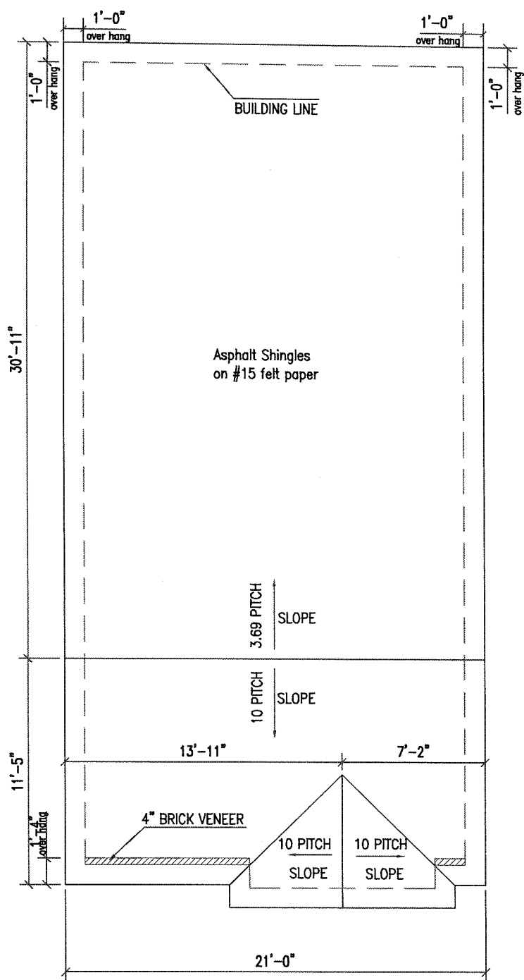
ROOF PLAN 6002 CLAY ST NE
