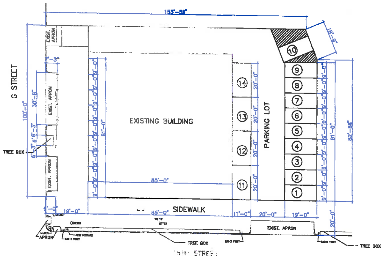
SITE PLAN FOR 702 15TH STREET, NE SCALE: 1" = 20'
