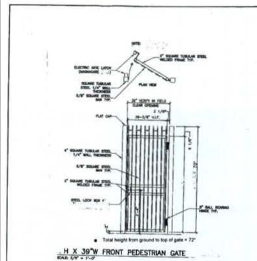
IRON PEDESTRIAN GATE DETAIL (TYP)
