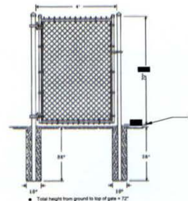
CHAINLINK GATE DETAIL (TYP)
