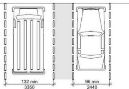
Fig. 502.2 Vehicle Parking Space Size
