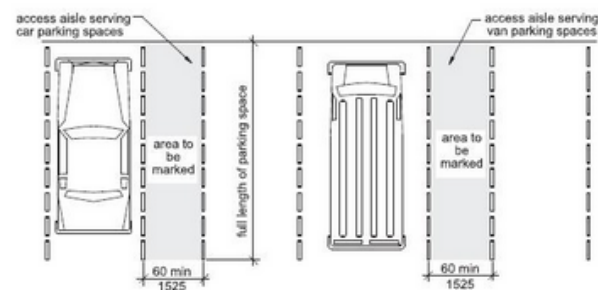
Fig. 502.4 Parking Space Access Aisle
