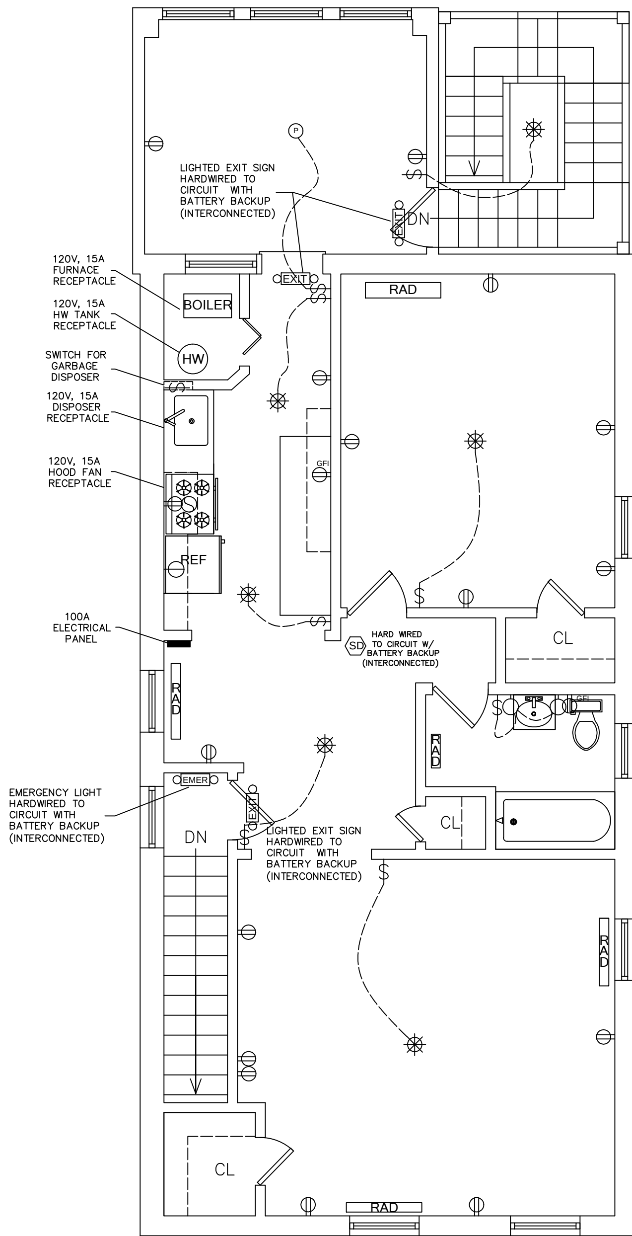
2ND FLOOR - ELECTRICAL SCALE: 1/4" = 1'-0"
