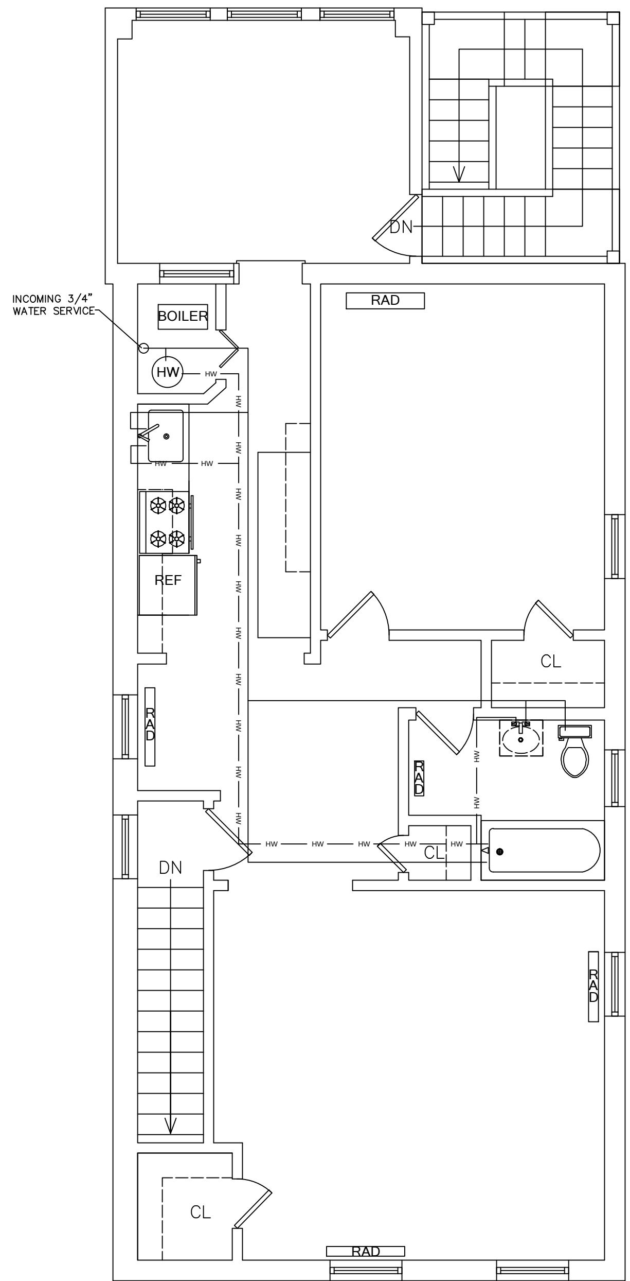
2ND FLOOR - PLUMBING SCALE: 1/4" = 1'-0"
