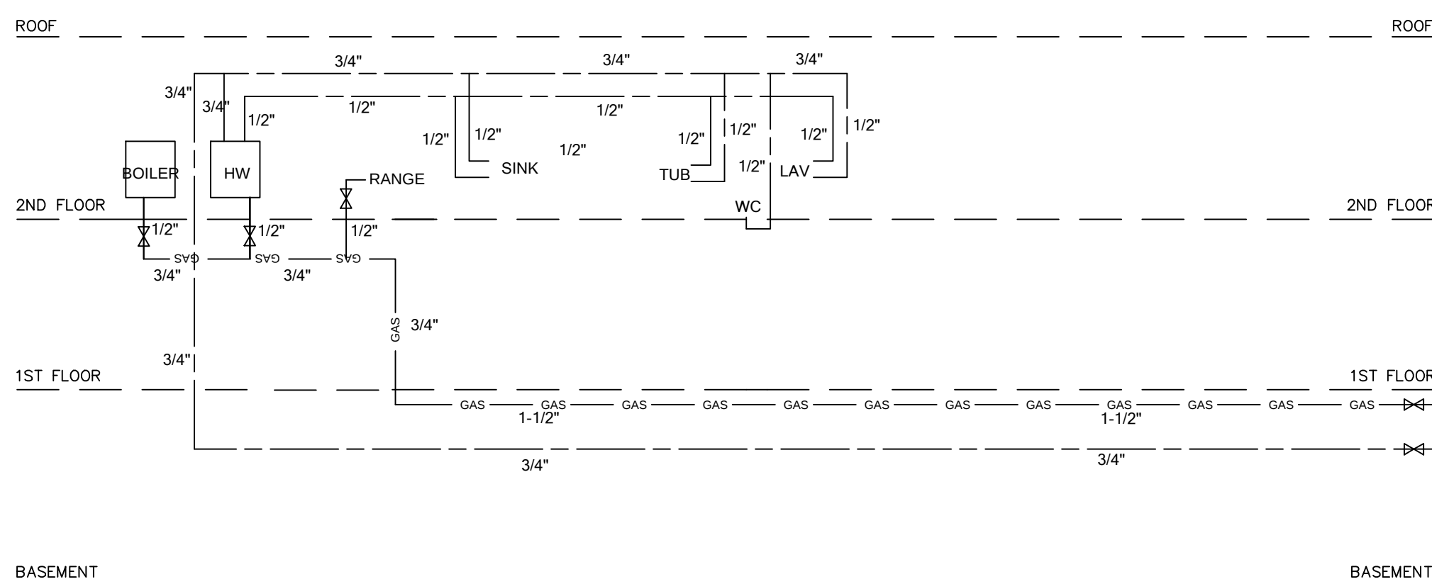
DOMESTIC RISER DIAGRAM SCALE: NO SCALE
