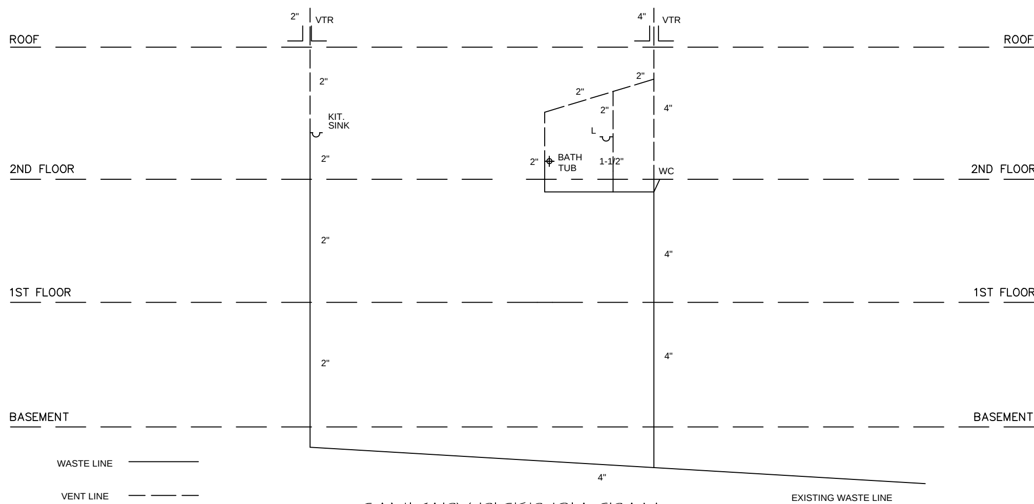
SANITARY RISER DIAGRAM SCALE: NO SCALE
