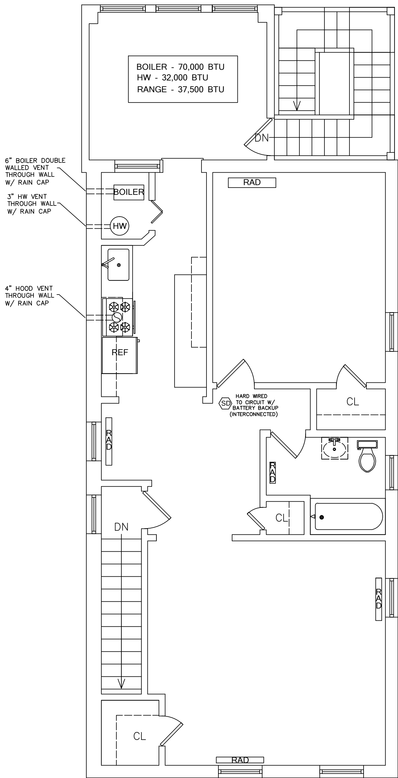
2ND FLOOR - MECHANICAL SCALE: 1/4" = 1'-0"
