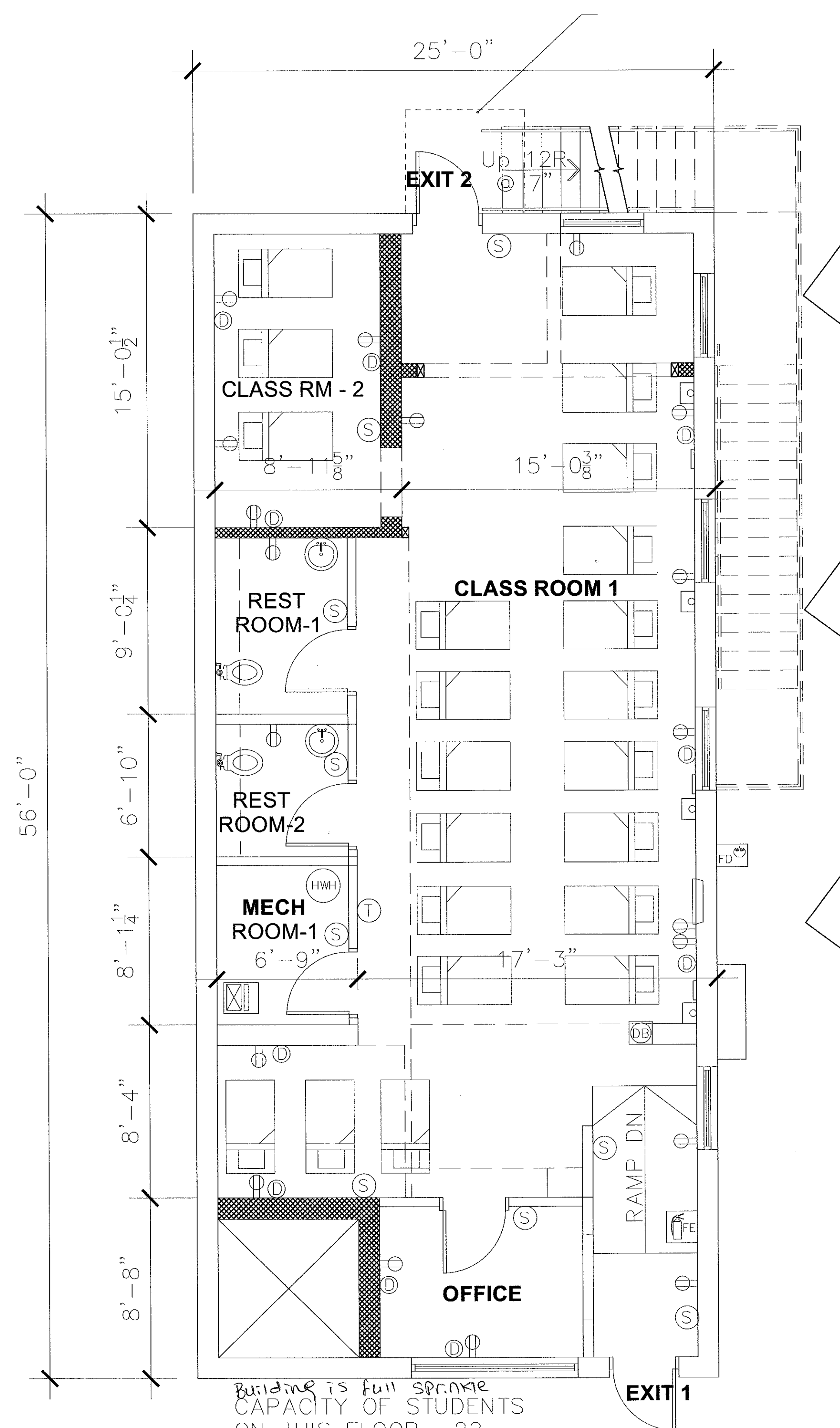
PLAN - GROUND FLOOR
