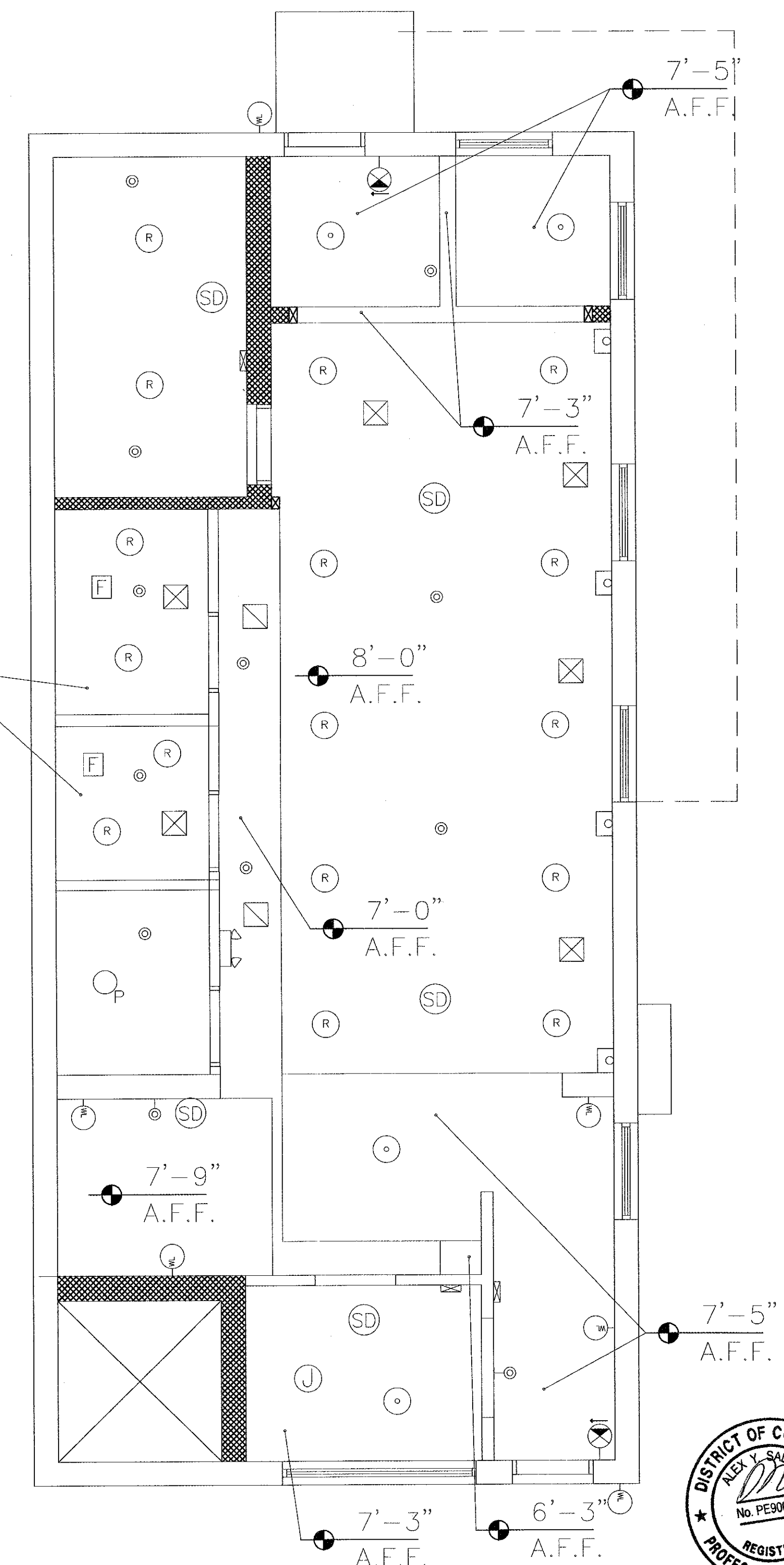
REFLECTED CEILING PLAN -GROUND FLOOR
