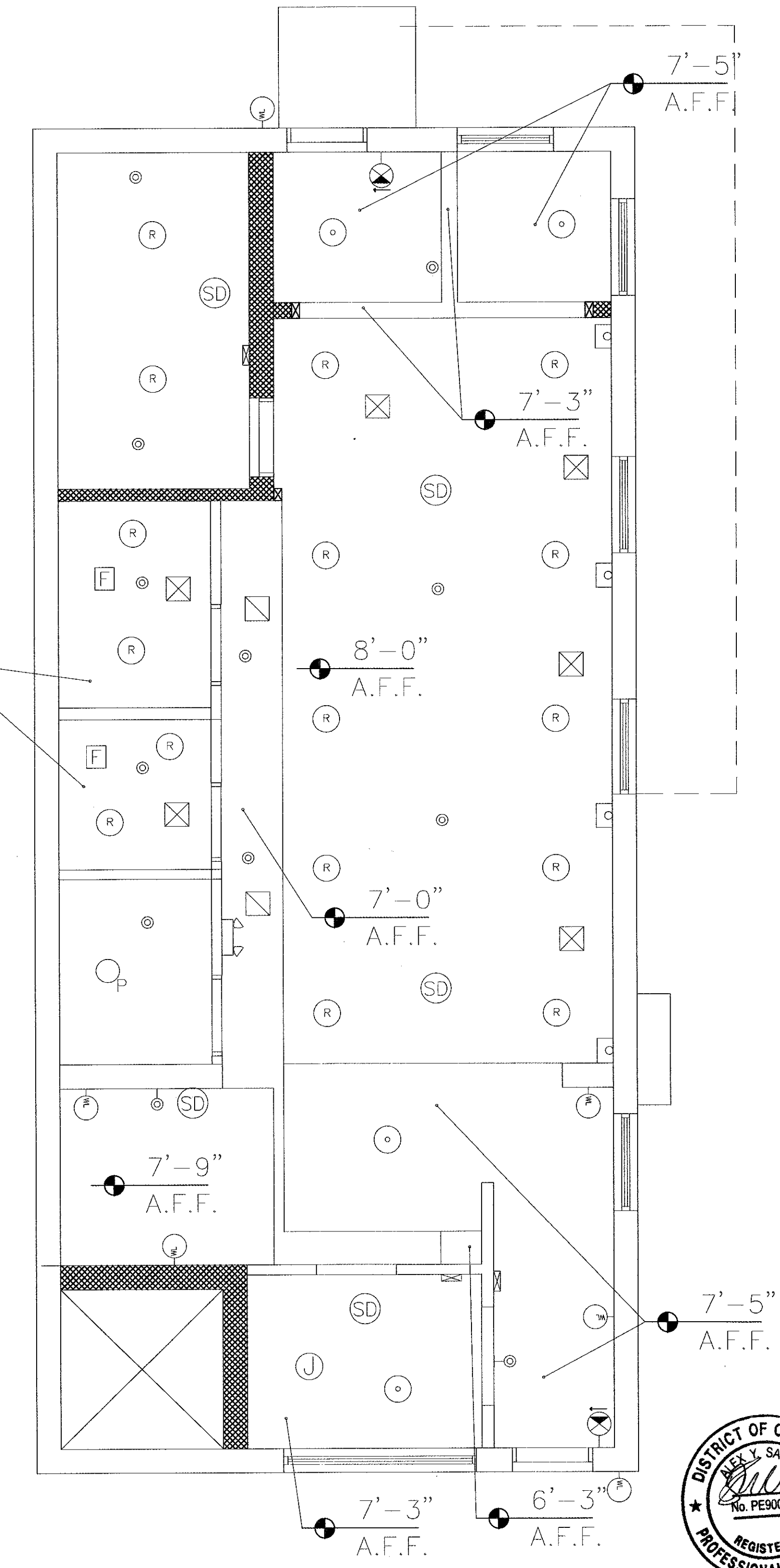
REFLECTED CEILING PLAN -GROUND FLOOR Scale: 1/4" = 1'
