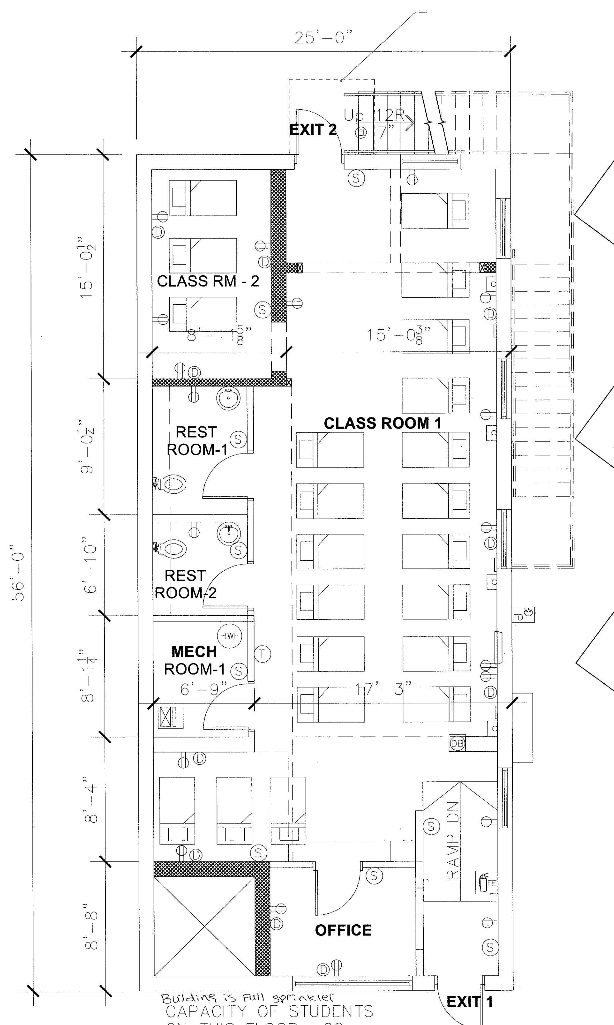
PLAN - GROUND FLOOR Scale: 1/4" = 1'
