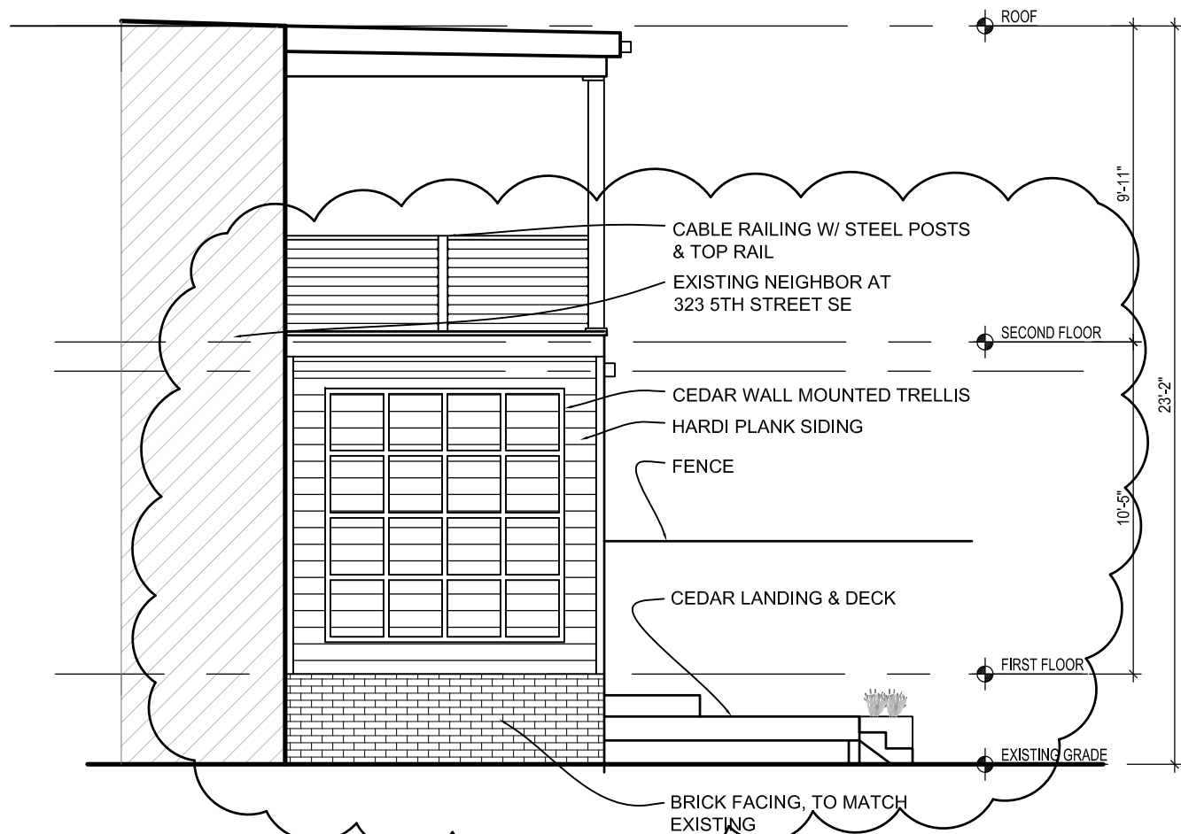
2 NORTH ELEVATION A-4 SCALE: 3/16"=1'-0"
