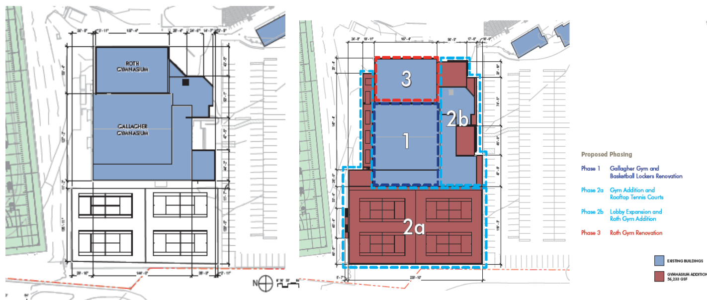
Existing First Floor Plan (Exhibit #11 Page 8)
