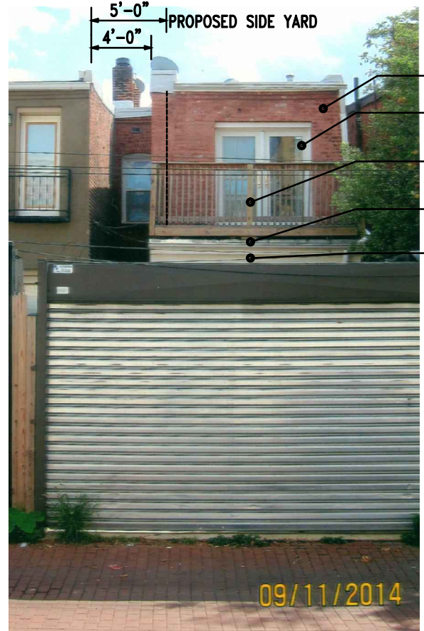
VIEW 2 REAR ELEVATION
