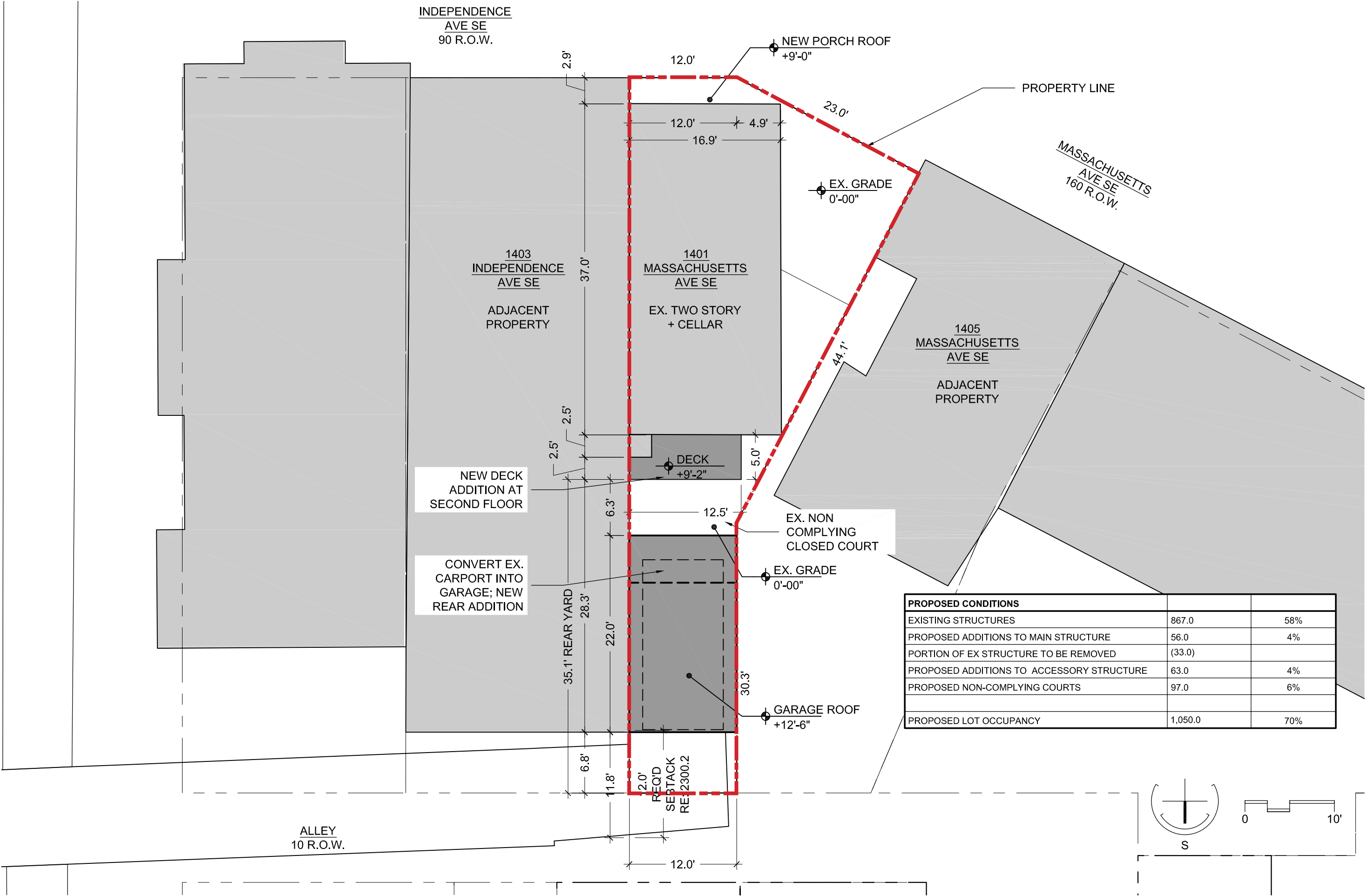
proposed site plan 1" = 10'-0"
