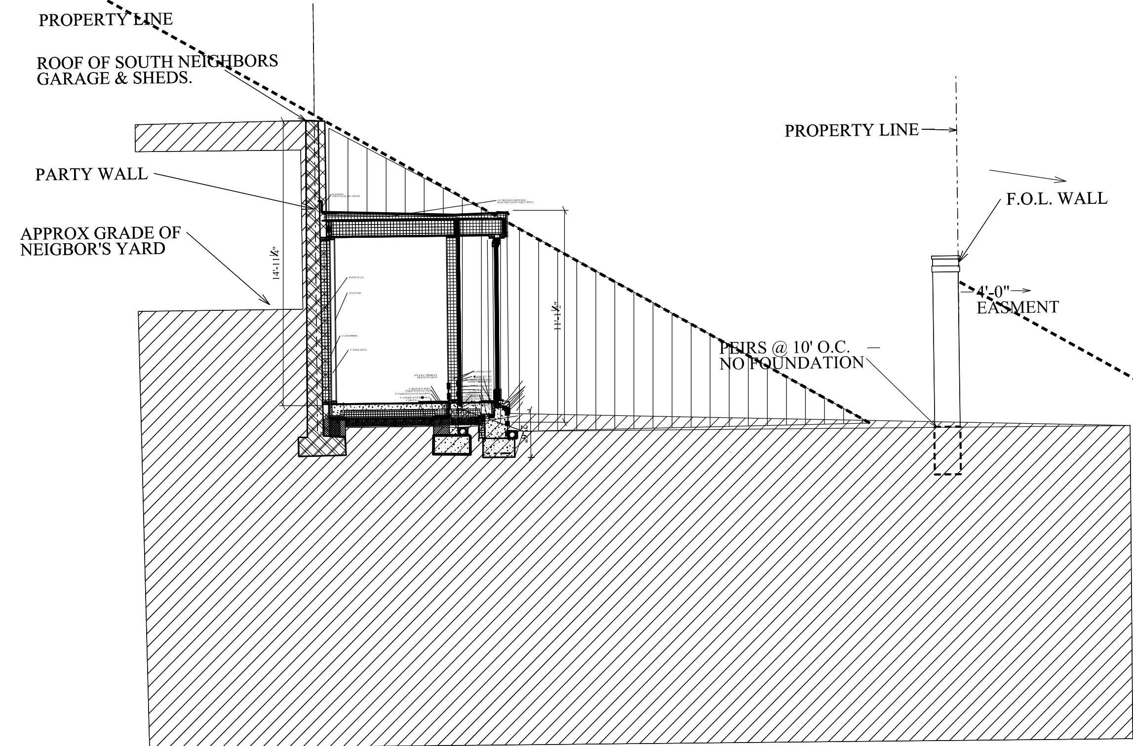
SUN ANGLE 29 deg WINTER SOLSTICE SECTION ILLUSTRATION
