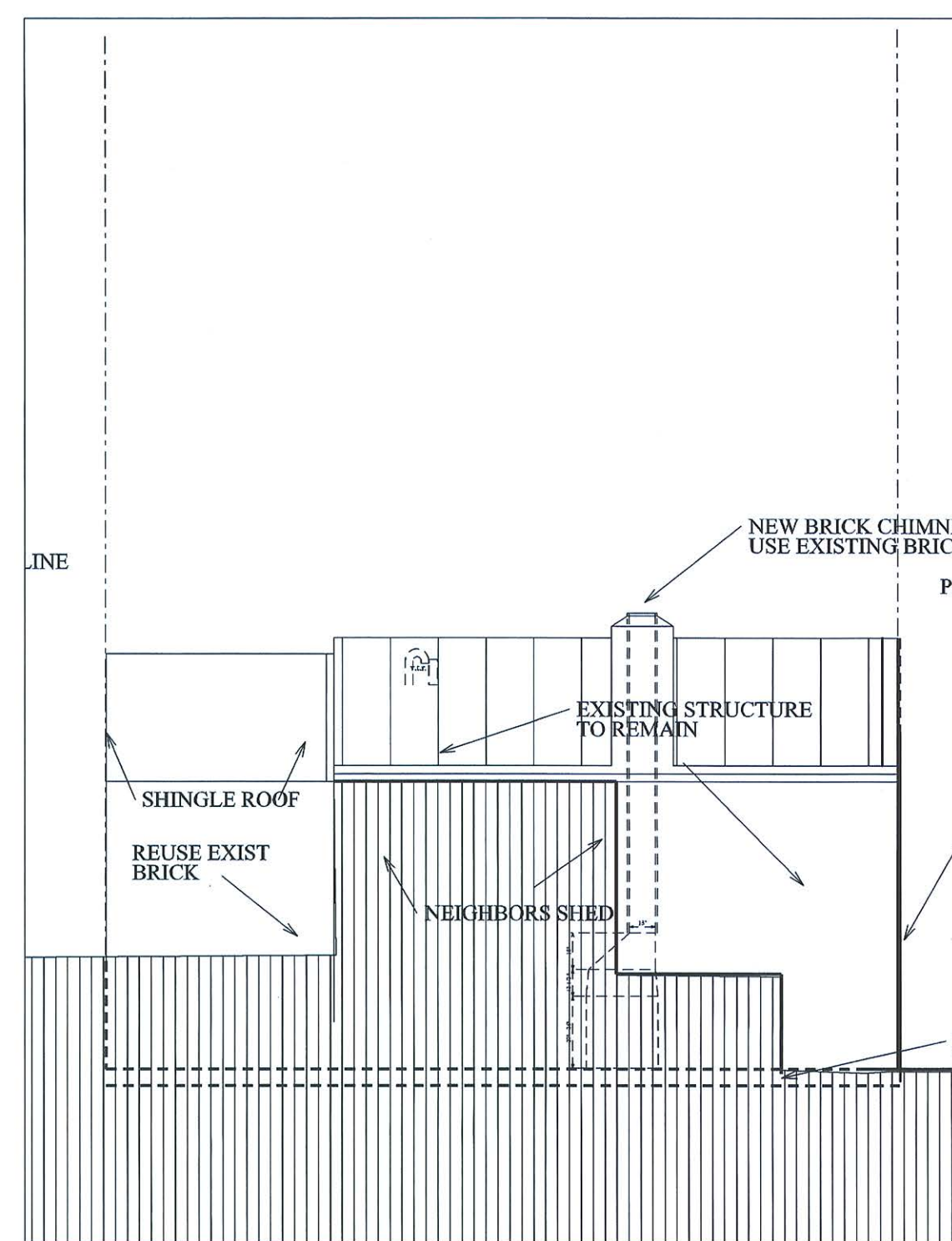
EAST GARAGE ELEVATION
