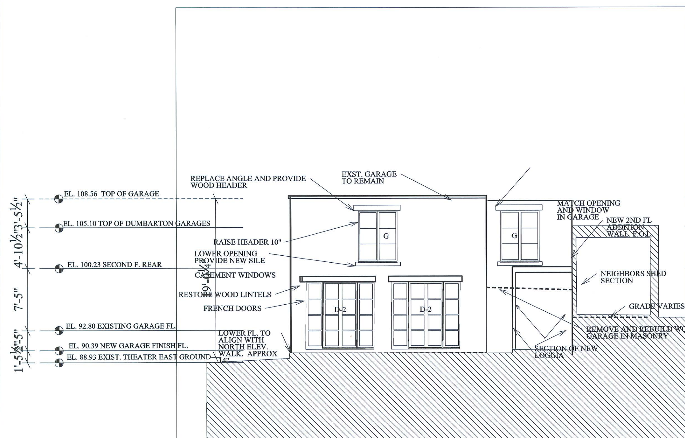
WEST CARRIAGE HOUSE ELEVATION
