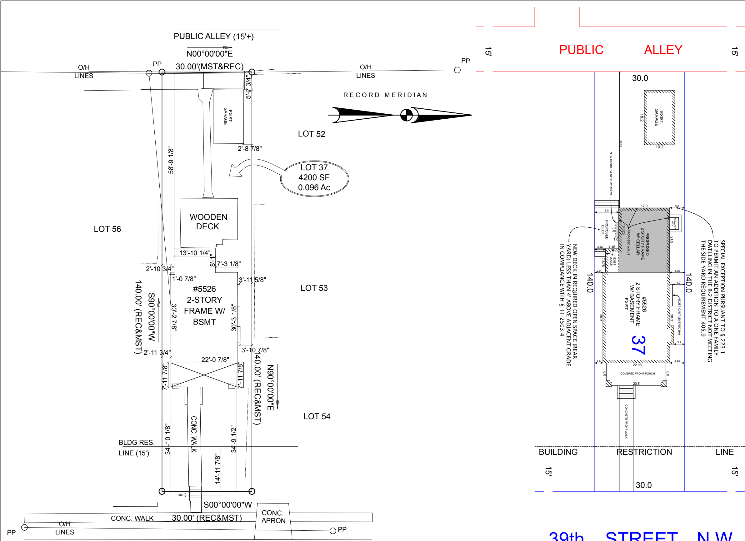
1 Existing Survey 1" = 20'
