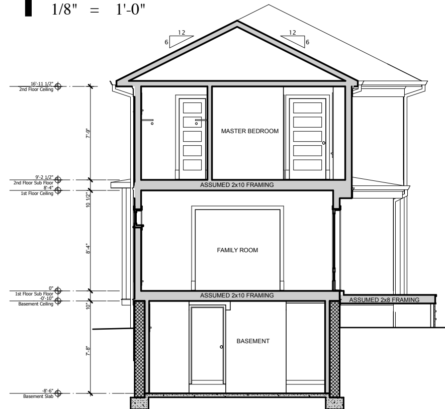
2 Building Section 2 1/8" = 1'-0"
