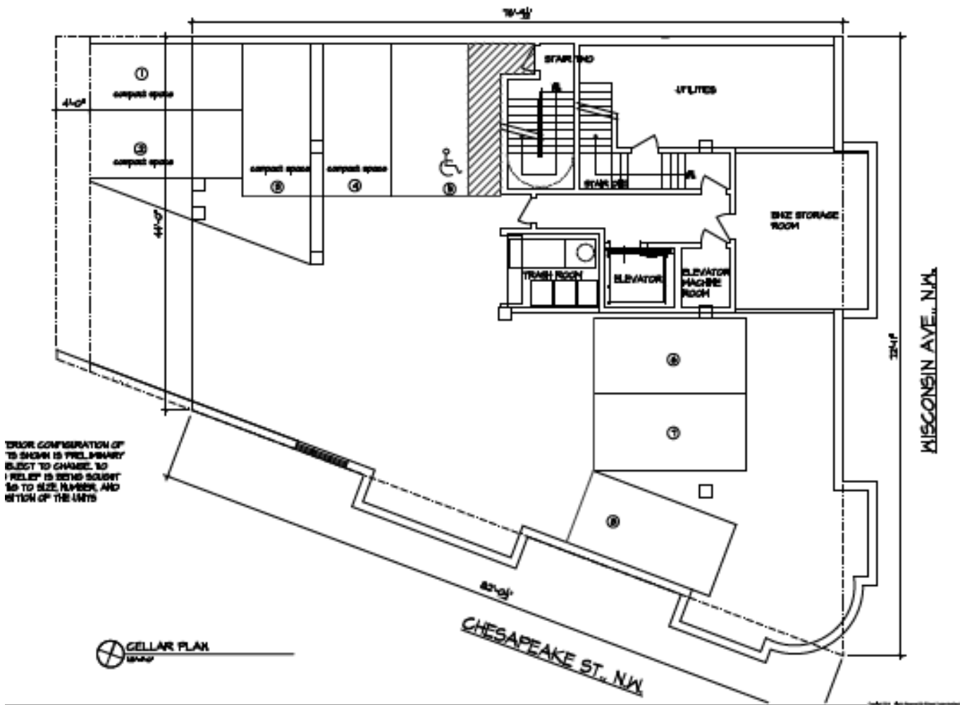
Figure 2. Basement and Parking Level
