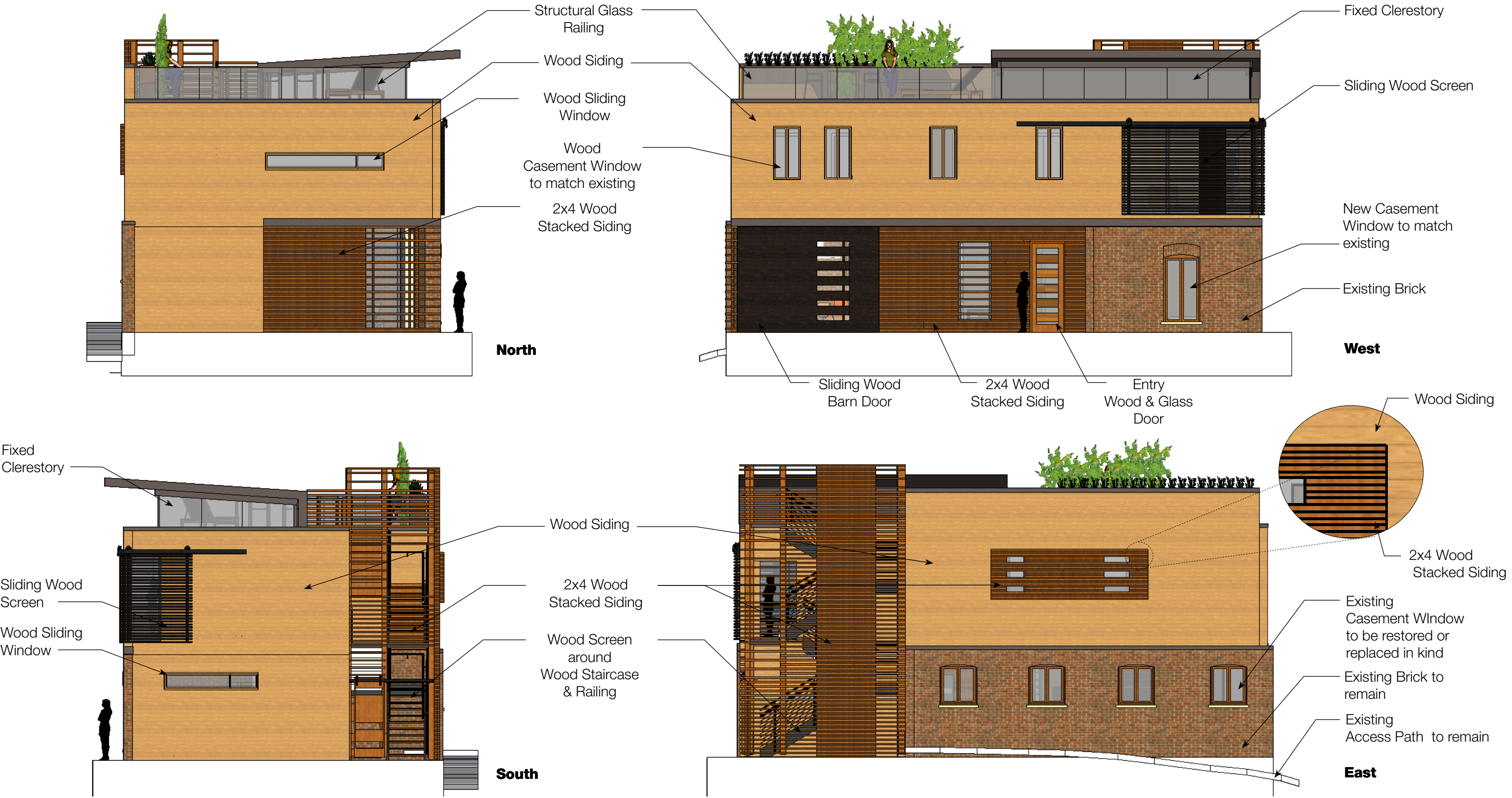
Exterior Elevations - Closed - 1/8" = 1'-0"
