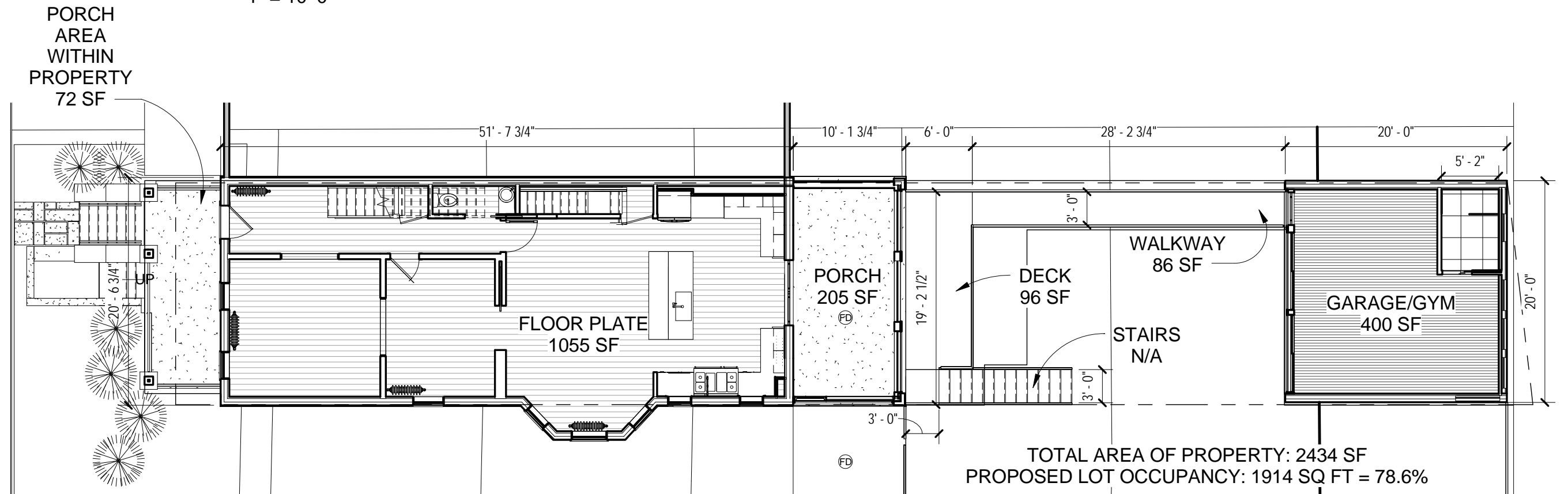
1 Z-1ST FLOOR PLAN 1" = 10'-0"
