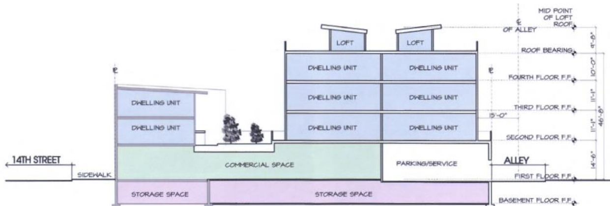
Figure 1. Proposed Section from North
