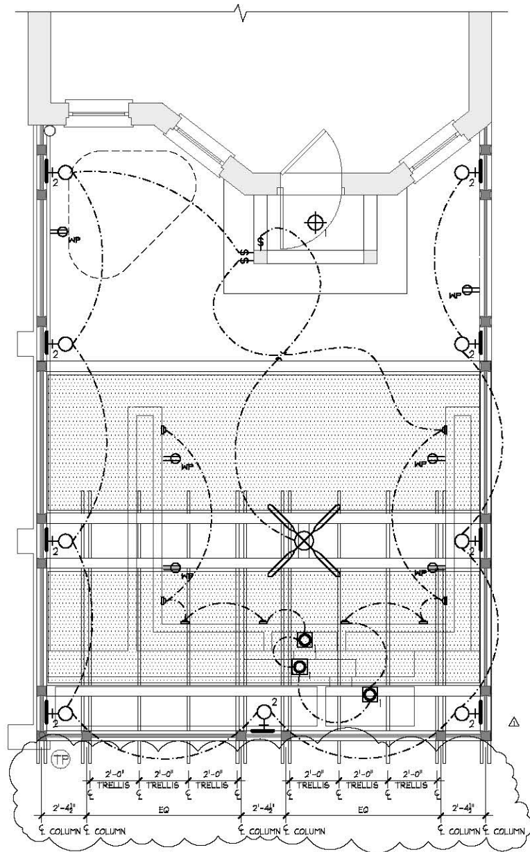
1 REFLECTED CEILING PLAN - DECK 3/8" = 1'-0"
