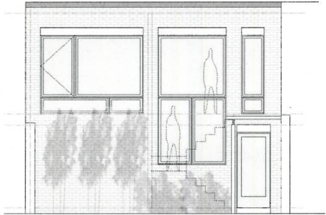
Proposed Rear Addition South Elevation (at Cityd.) scale: 1/8" = 1'-0"
