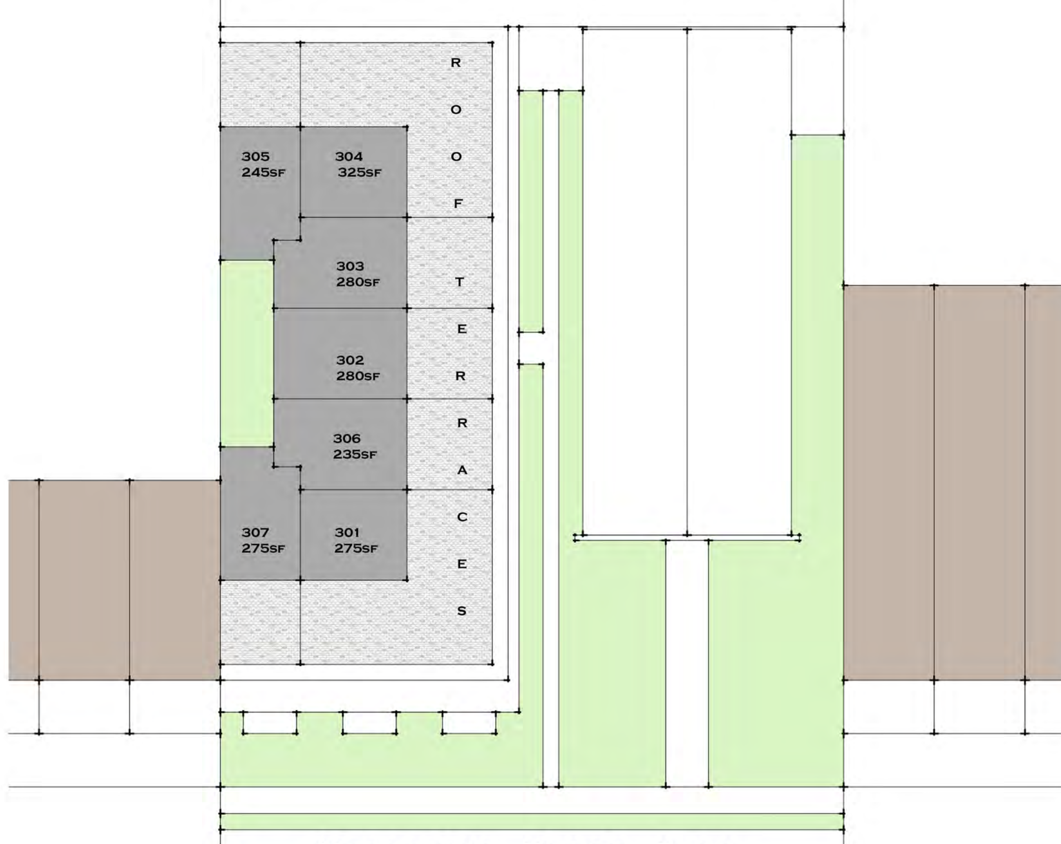
MEZZANINE FLOOR PLAN
