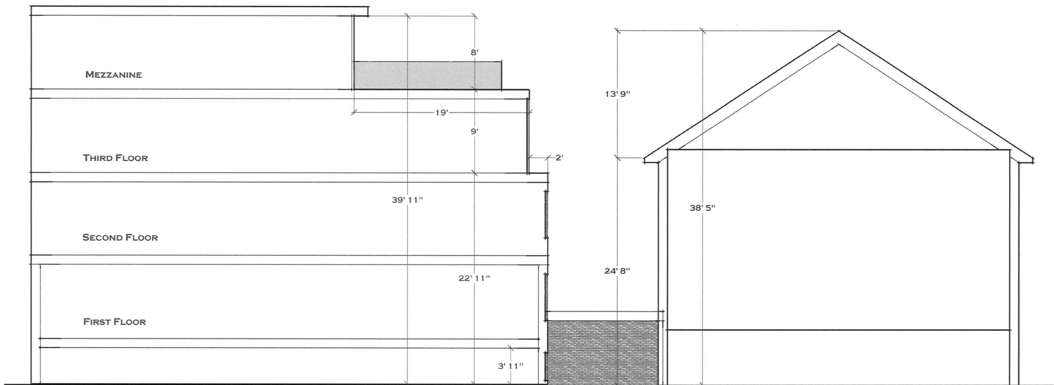
SECTION THRU BUILDING
