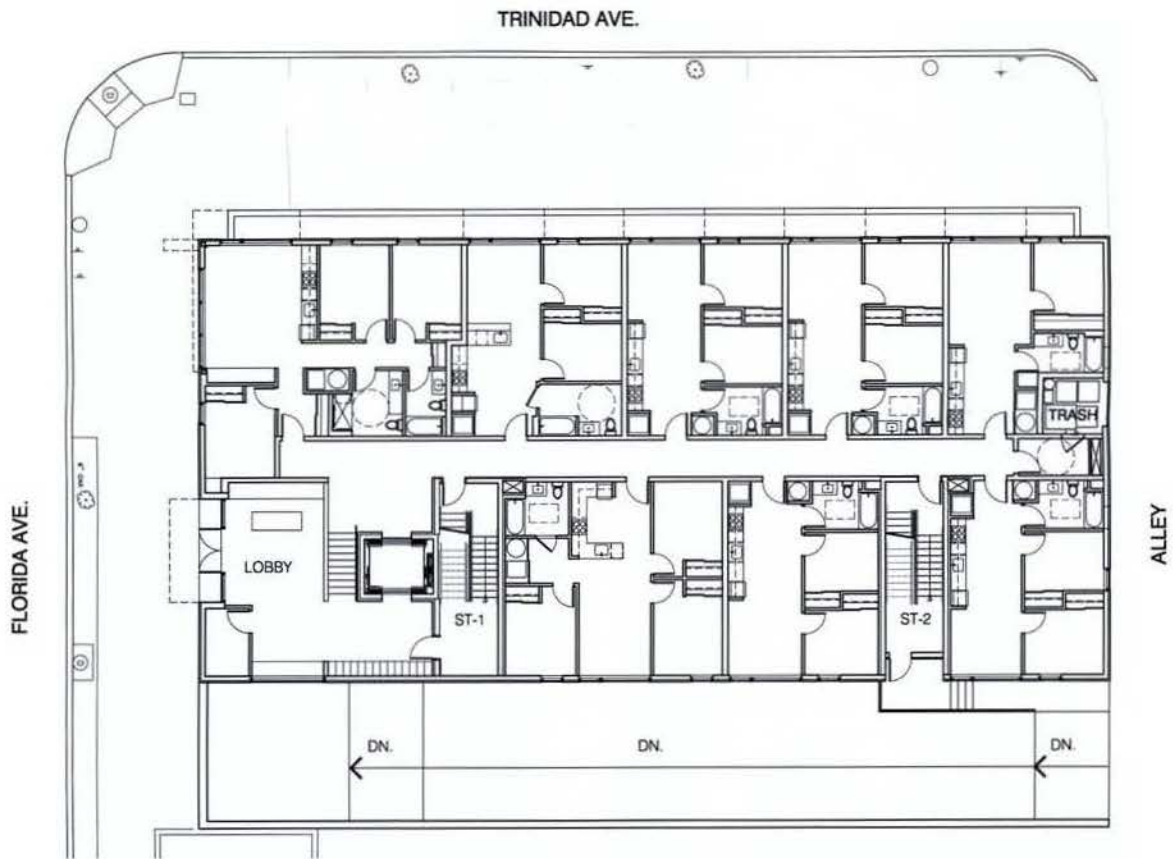
GROUND FLOOR PLAN 1/16"=1'-0"
