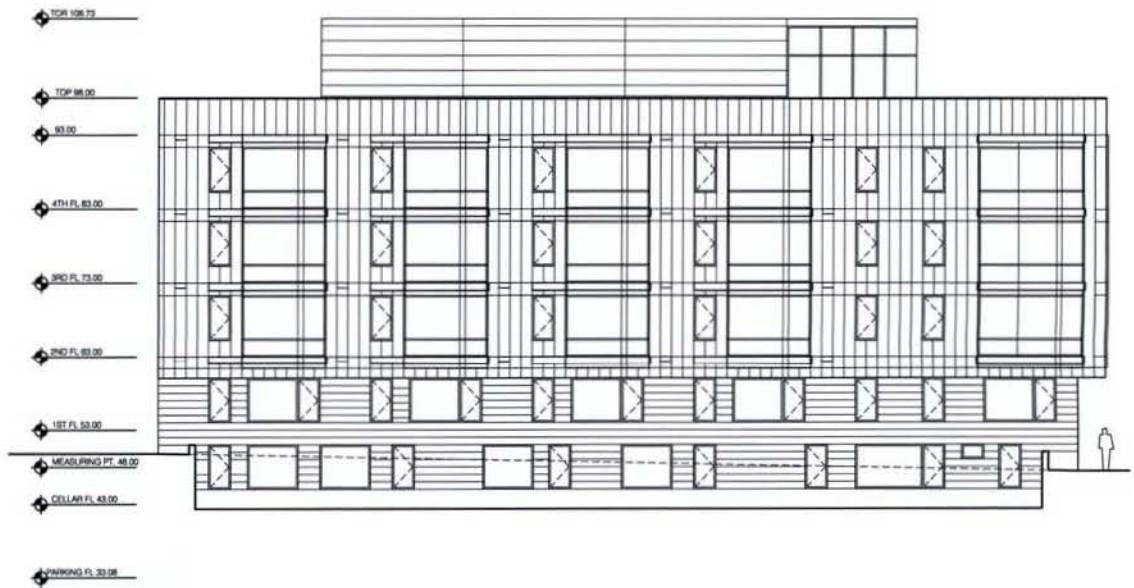
WEST ELEVATION - TRINIDAD STREET 1/16"=1'-0"
