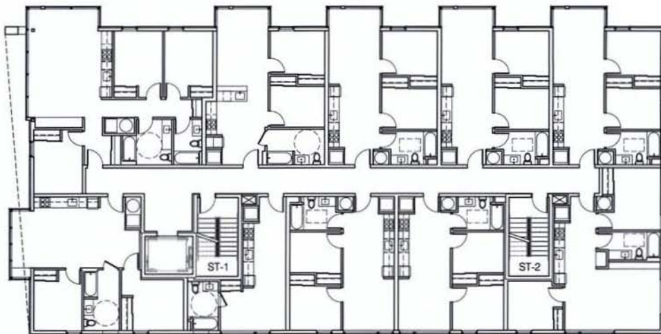
4TH FLOOR PLAN 1/16"=1'-0"
