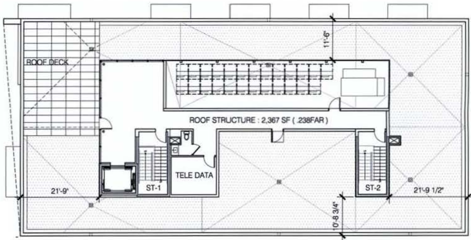
ROOF PLAN 1/16"=1'-0"
