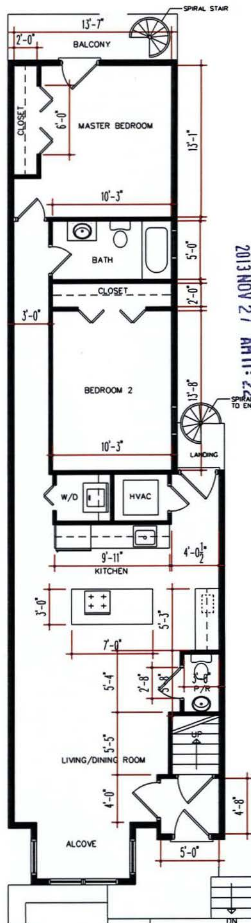
PROPOSED 1st FLOOR
