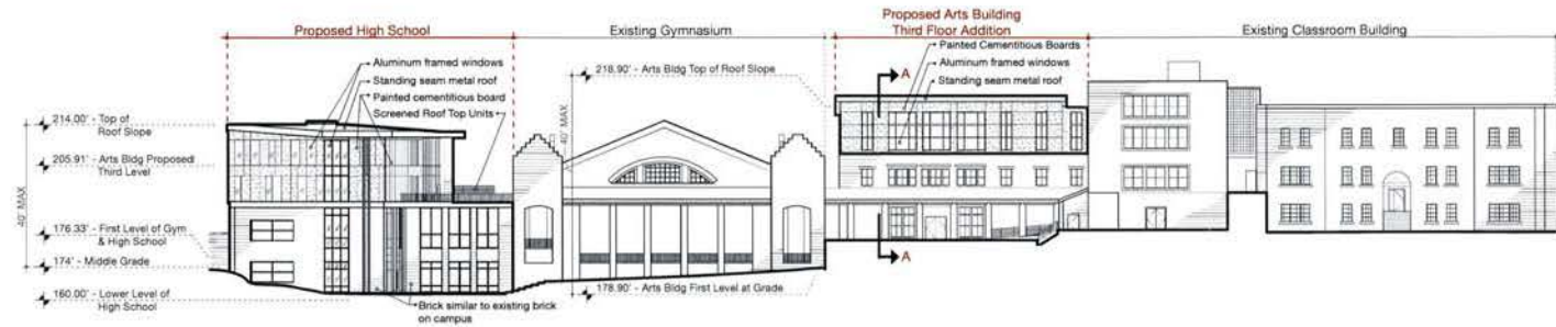
Elevation 1 Behind Castle & Carriage House scale: 1" = 60'-0"
