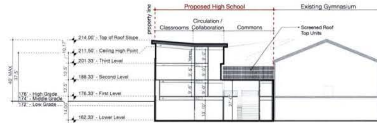
Section B-B - Proposed High School at Commons scale: 1" = 60'-0"
