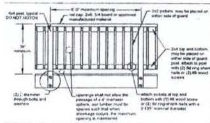
Deck Railing Detail
