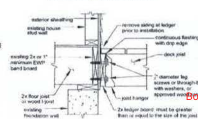
Ledger Attachment Detail
