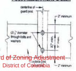
Post Attachment Detail
