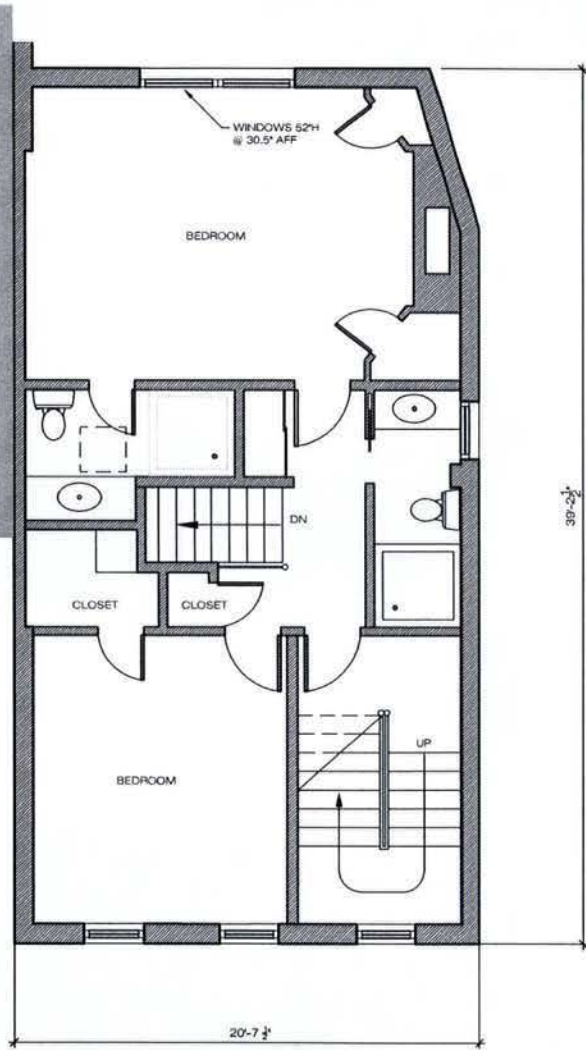
01 2ND FLOOR PLAN NEW WORK SCALE: 3/16" = 1'-0"
