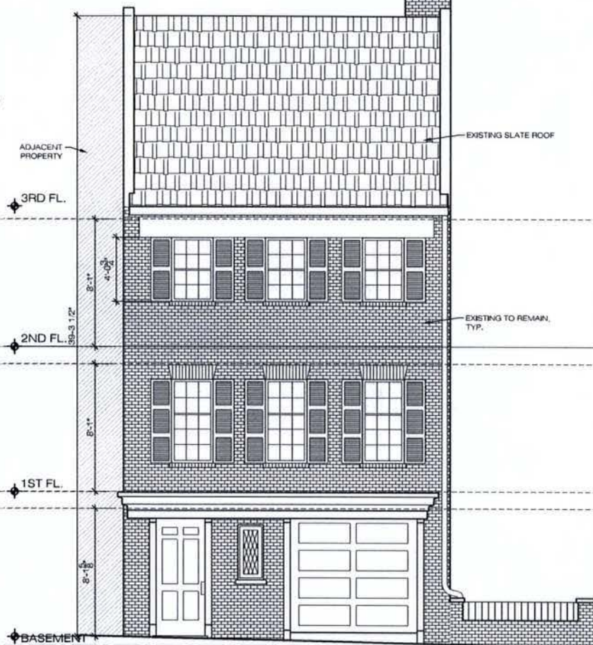
02 SOUTH ELEVATION (FRONT) SCALE: 3/16" = 1'-0"
