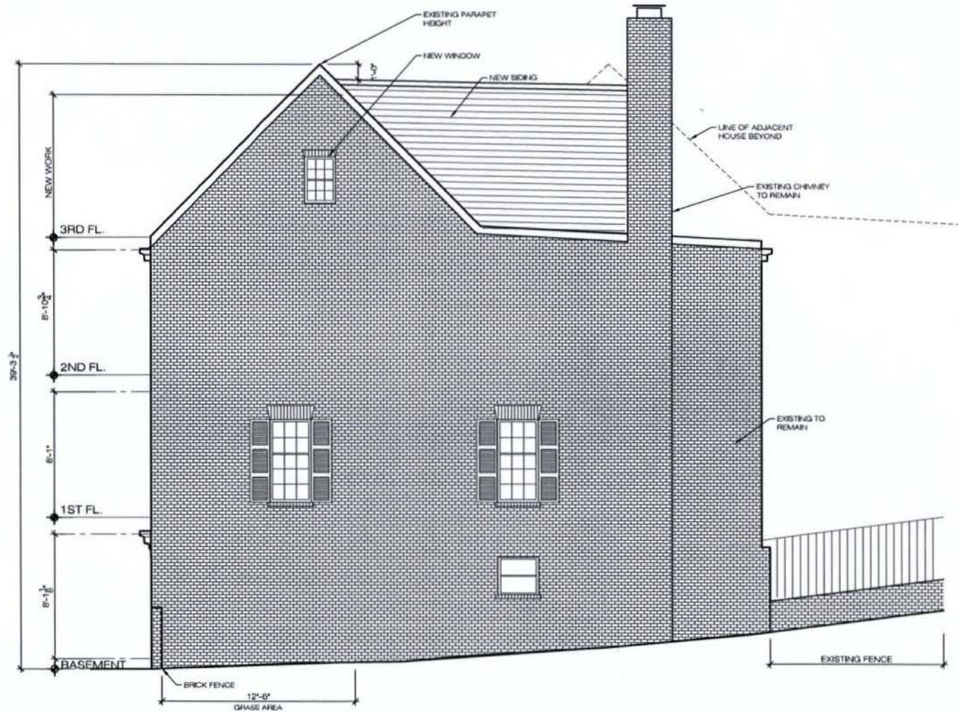
01 NEW WORK EAST ELEVATION SCALE: 3/16" = 1'-0"
