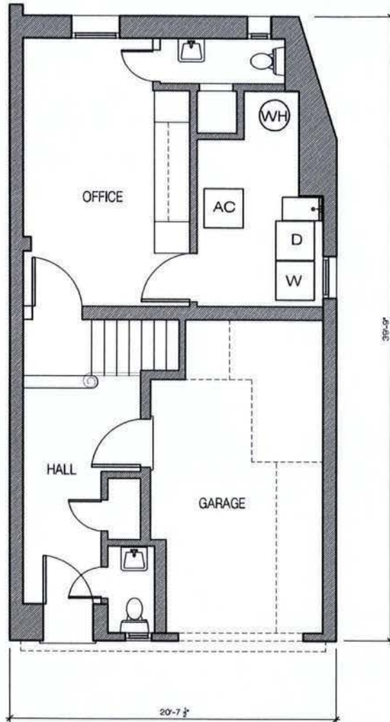
01 EXISTING BASEMENT FLOOR PLAN
