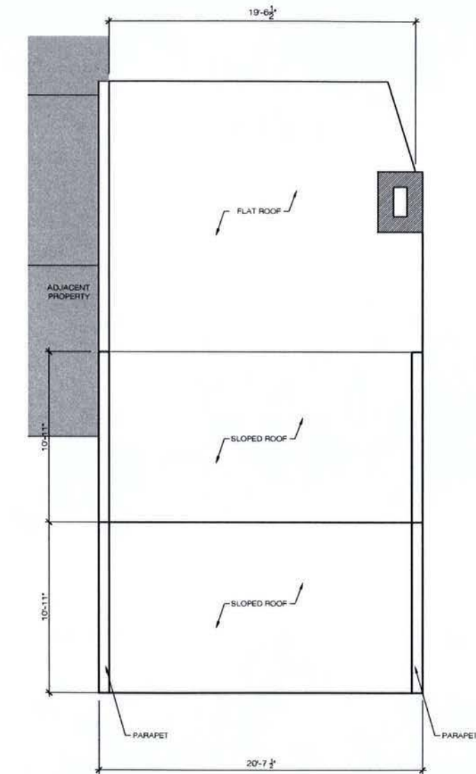
01 EXISTING ROOF PLAN SCALE: 3/16" = 1'-0"
