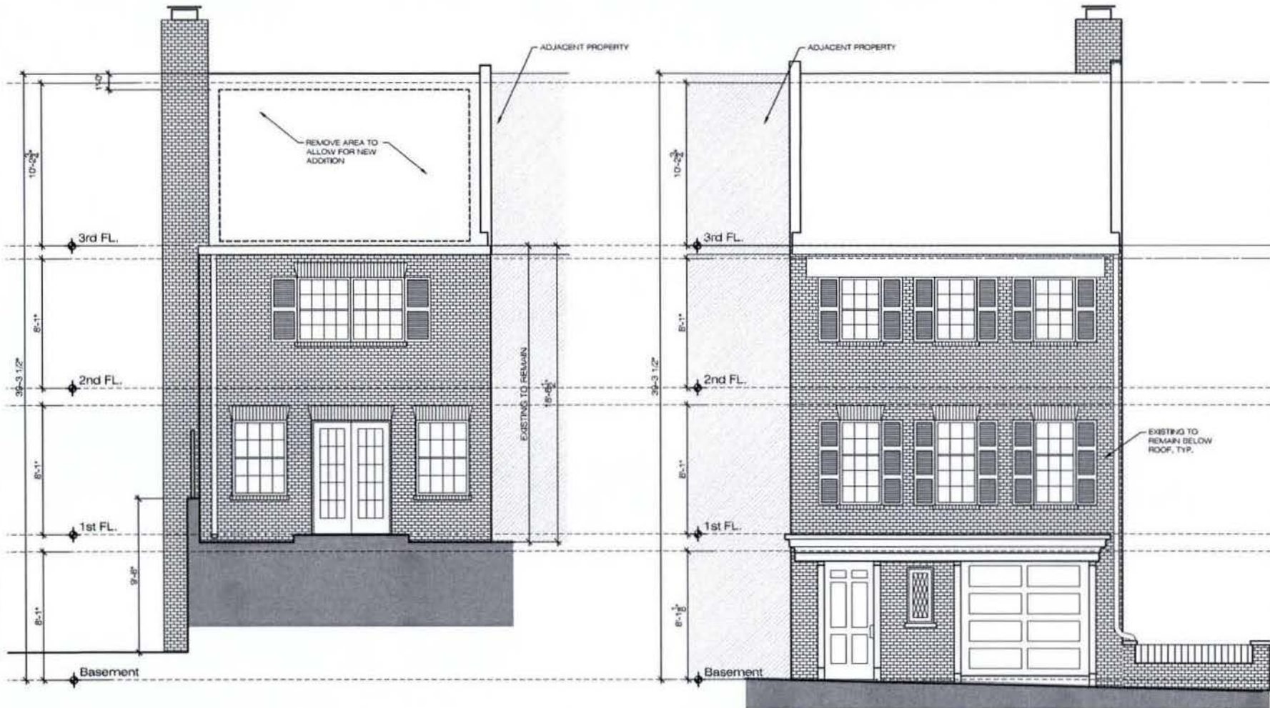
02 SOUTH ELEVATION (FRONT) SCALE: 3/16" = 1'-0"
