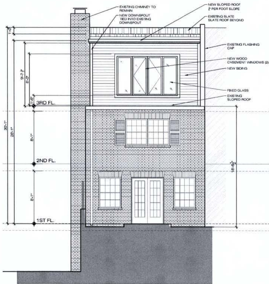
01 NORTH ELEVATION (REAR) SCALE: 3/16" = 1'-0"
