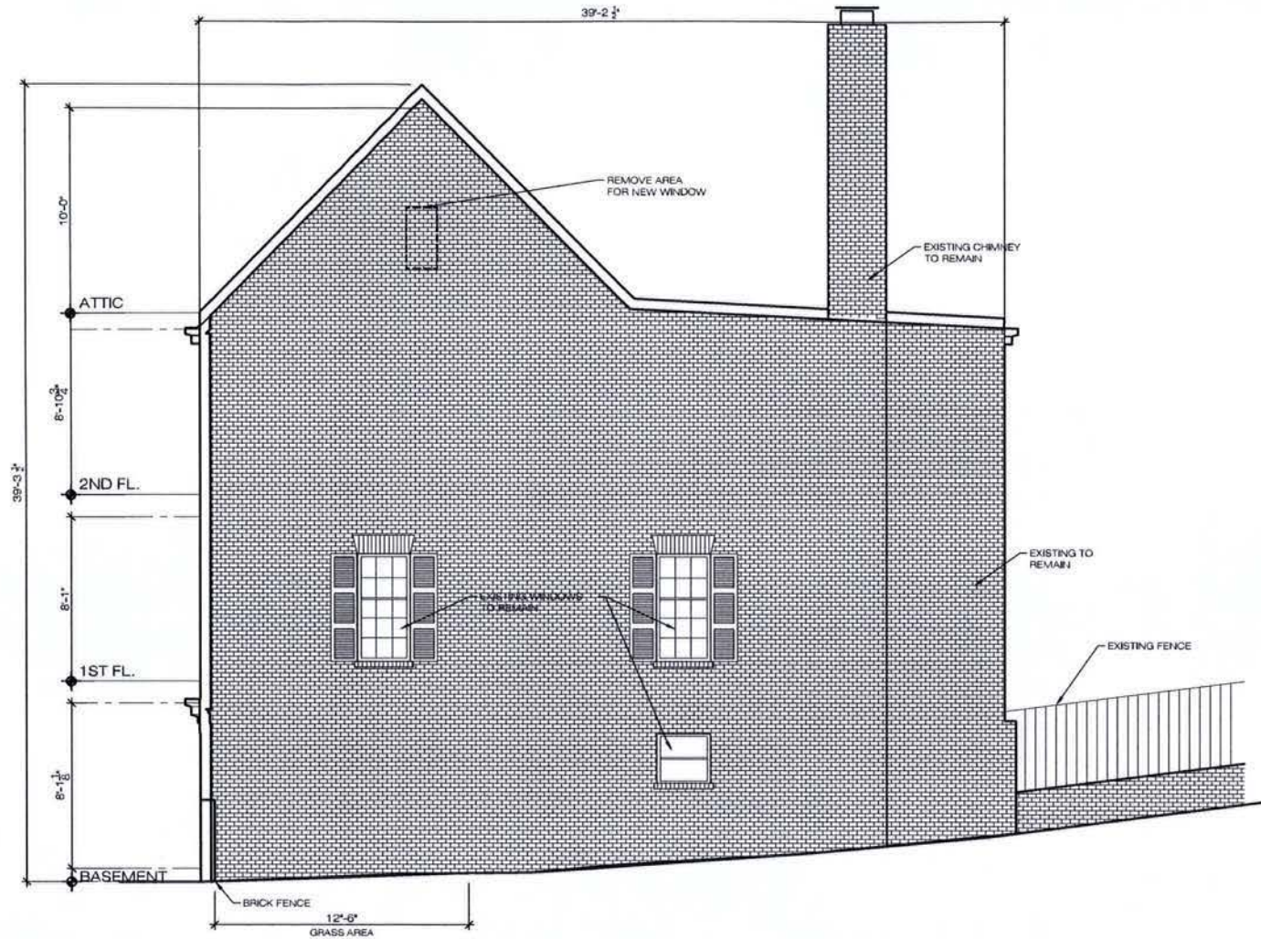
01 EXISTING EAST ELEVATION SCALE: 3/16" = 1'-0"
