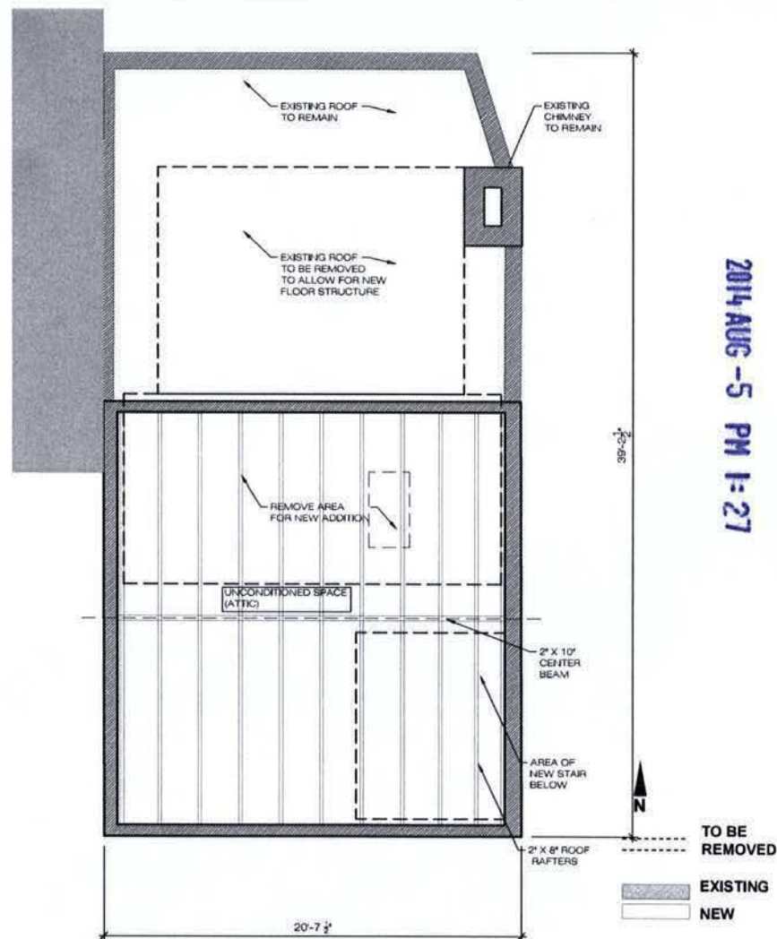
02 EXISTING ATTIC PLAN
