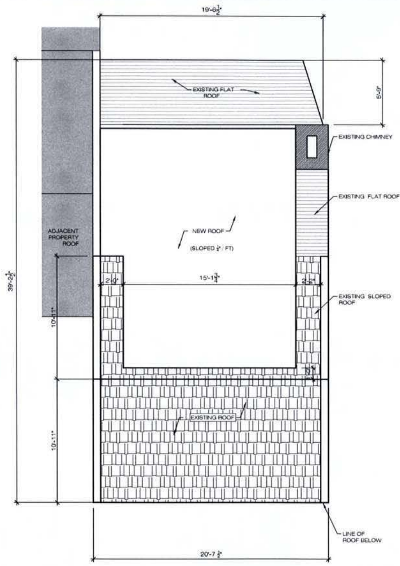
01 ROOF PLAN NEW WORK SCALE: 3/16" = 1'-0"
