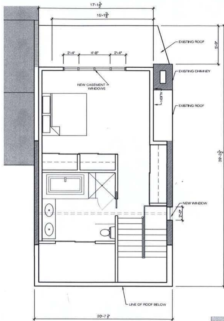
02 3RD FLOOR PLAN NEW WORK SCALE: 3/16" = 1'-0"
