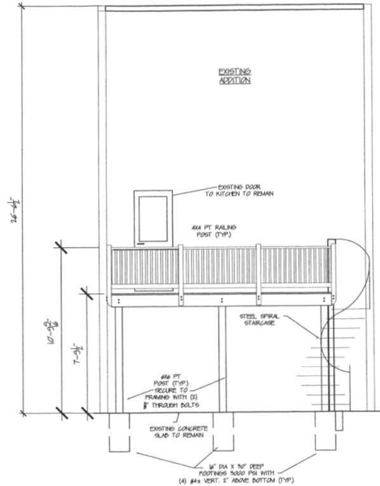
PROPOSED ELEVATION 1/4" = 1'-0"
