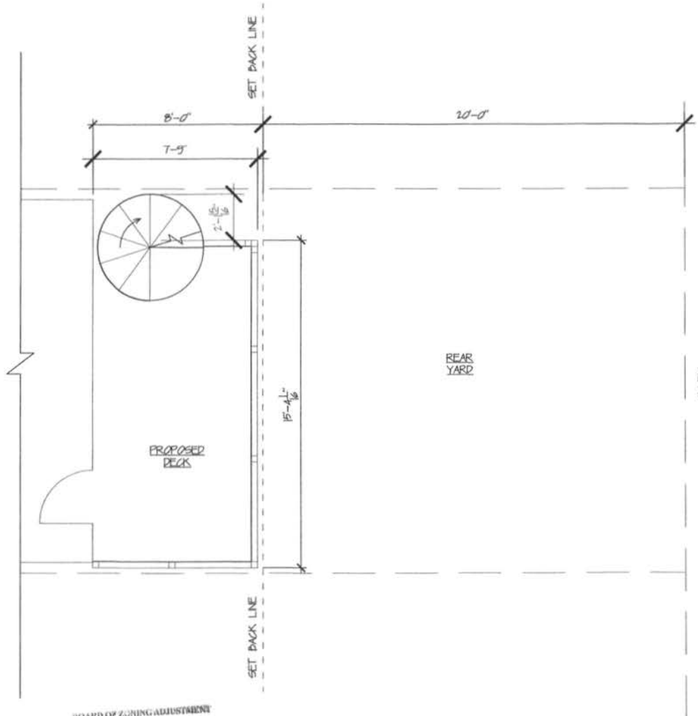
PROPOSED PLAN 1/4" = 1'-0"
