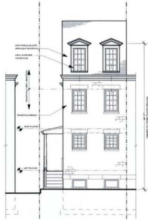
1 PROPOSED FRONT ELEVATION Scale: 1/4" = 1'-0"
