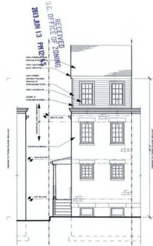
1 PROPOSED FRONT ELEVATION Scale: 1/4" = 1'-0"
