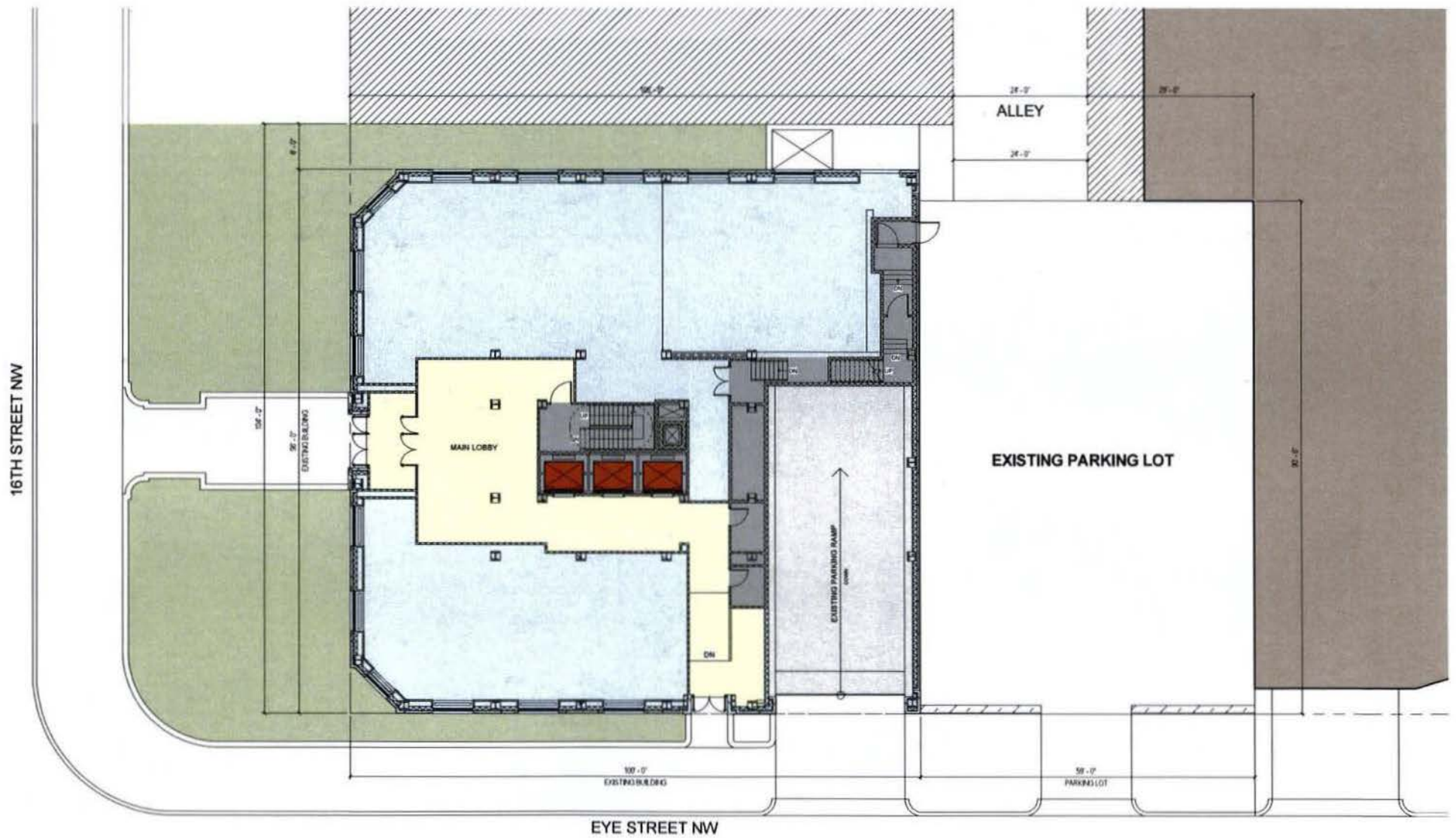
EXISTING SITE PLAN/GROUND FLOOR PLAN
