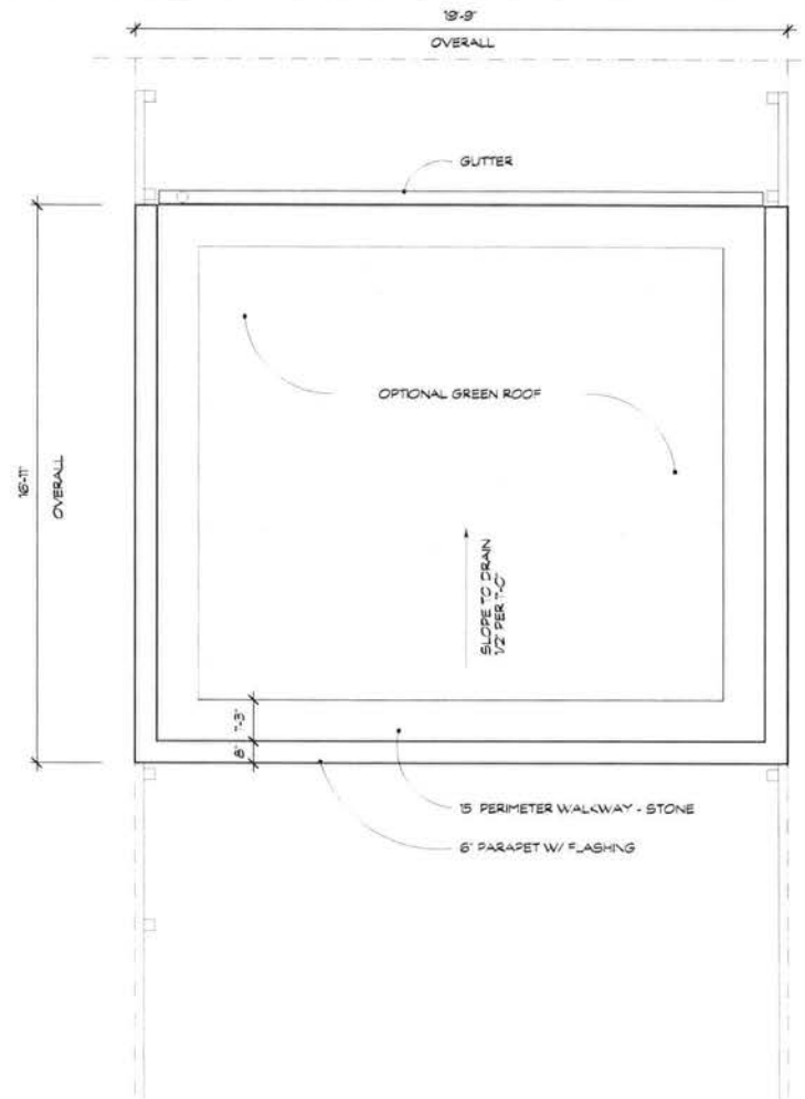
2 ROOF PLAN
