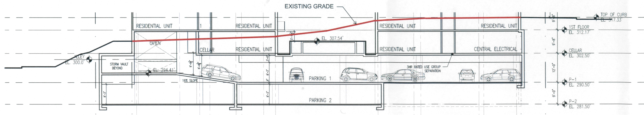
1 BUILDING SECTION
