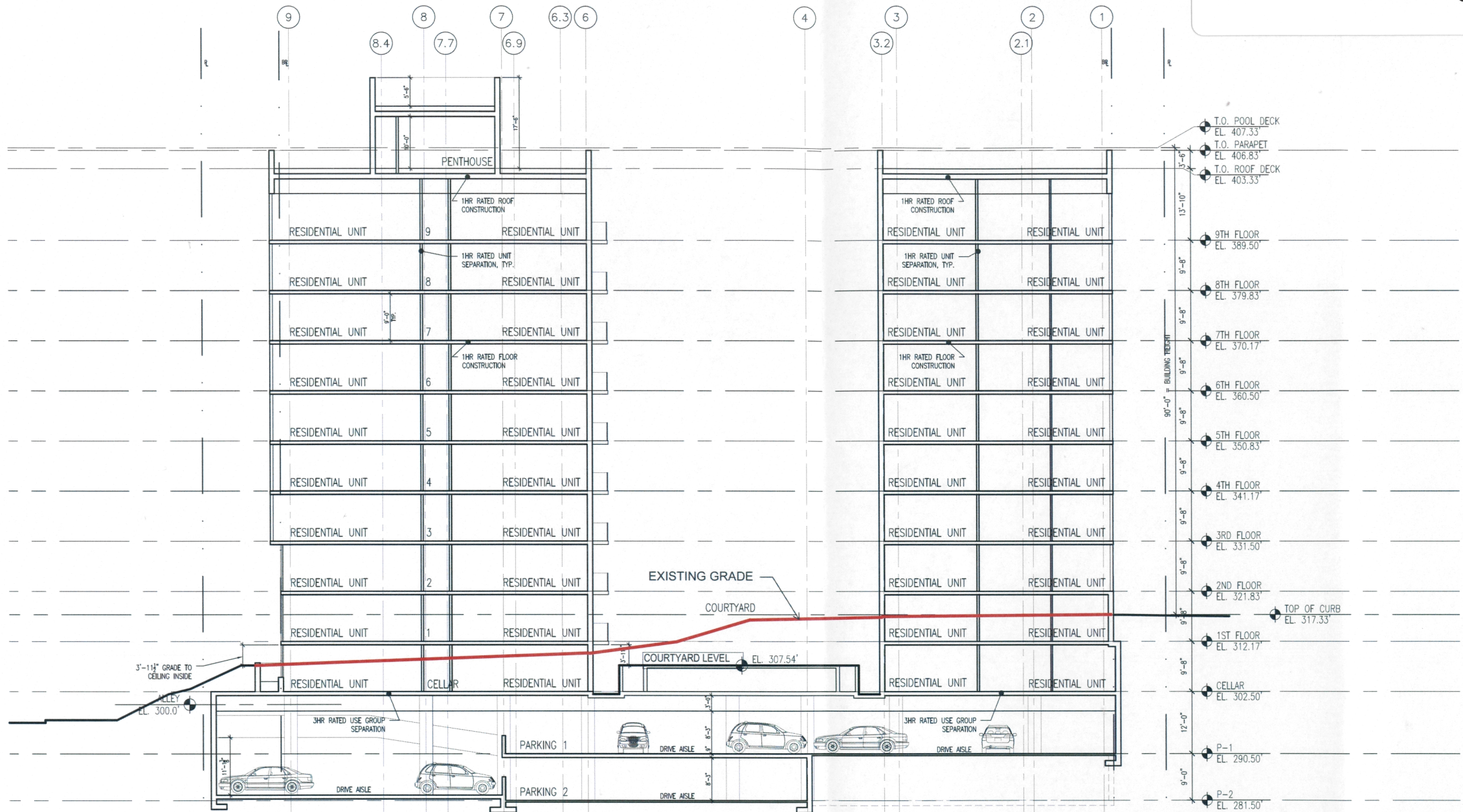
2 BUILDING SECTION
