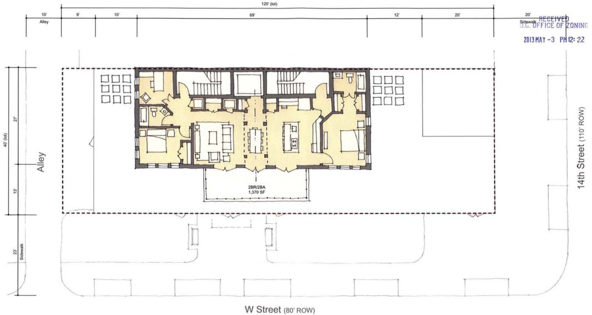
6th Floor Plan
