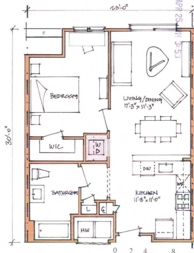
UNIT PLAN TYPE "B"
