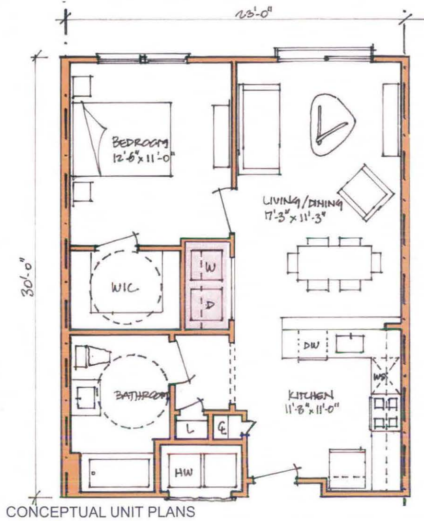
UNIT PLAN TYPE "A"
