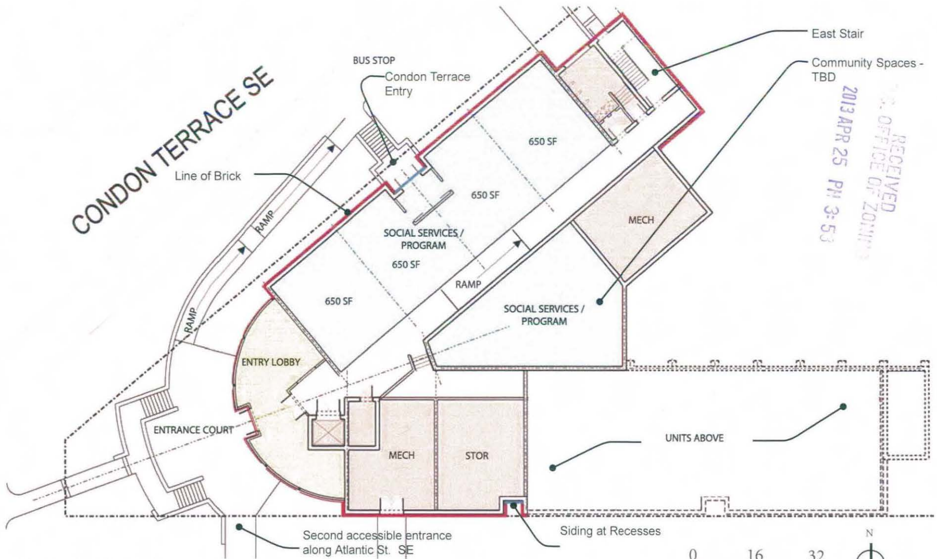
Building Plans: First Floor Plan
