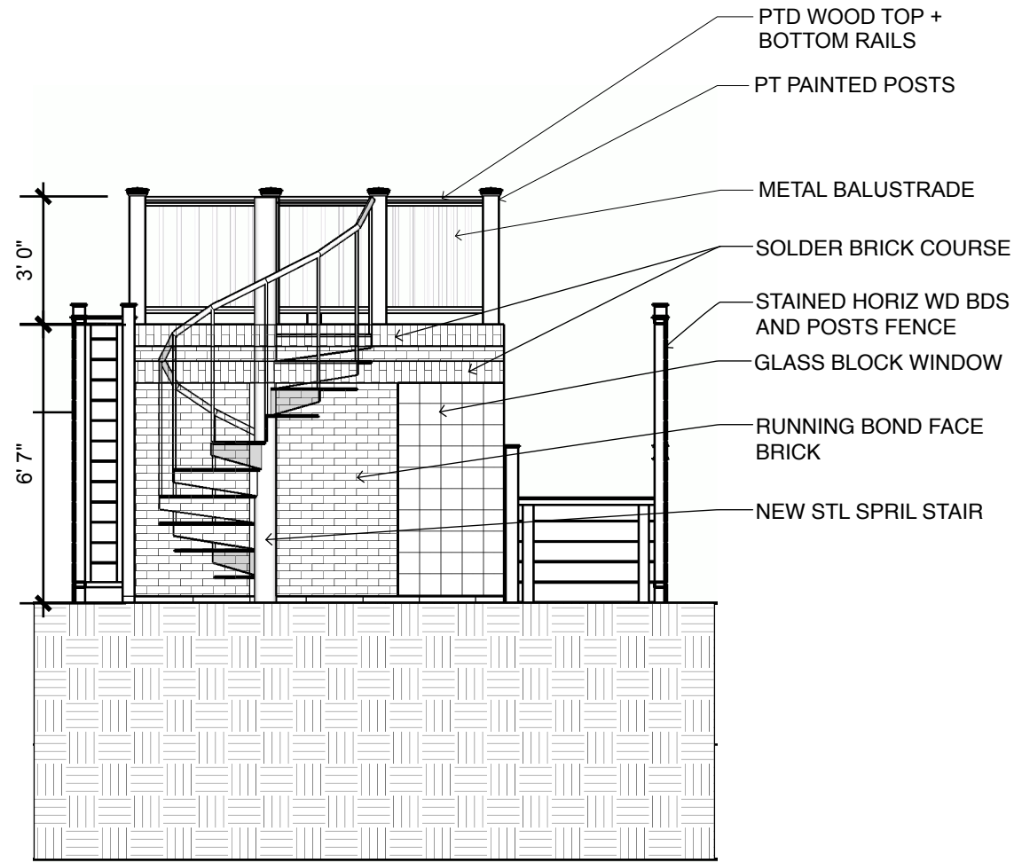
1 SOUTH ELEVATION Scale: 1/4" = 1'-0"
