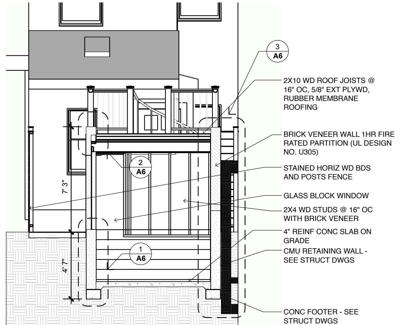
1 BUILDING SECTION Scale: 1/4" = 1'-0"
