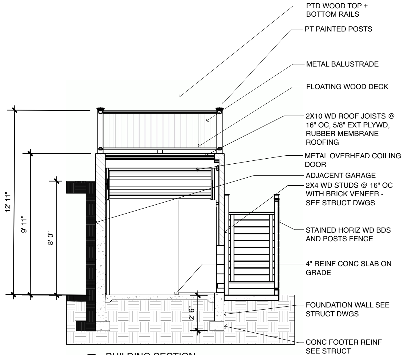
2 BUILDING SECTION Scale: 1/4" = 1'-0"
