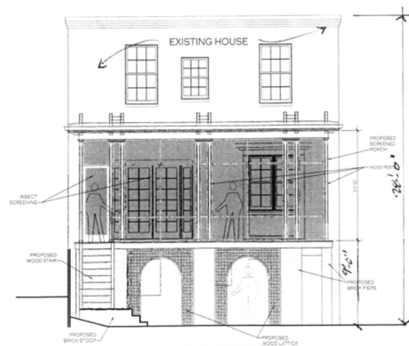
3 SOUTH ELEVATION SCALE: 1/4" = 1'-0"
