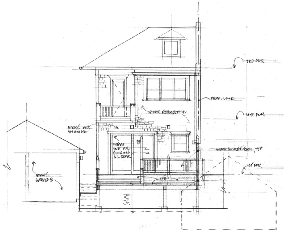
SOUTH ELEV. & SECT. B-B 1/4" = 1'-0"
