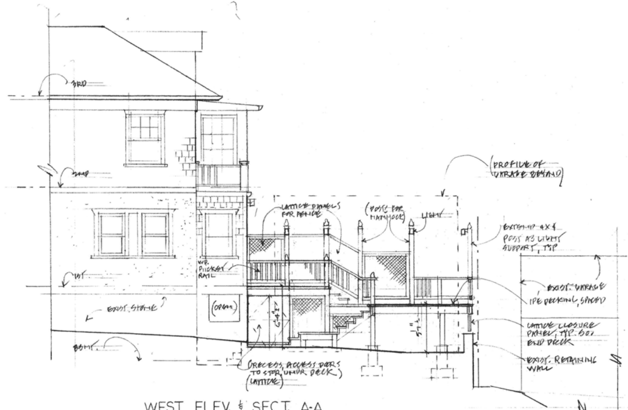
WEST ELEV. & SECT. A-A \frac{1}{4}" = 1'-0"
