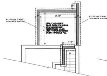
ADDITION FOUNDATION PLAN
