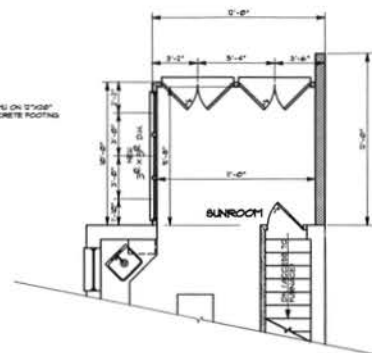
FIRST FLOOR ADDITION
