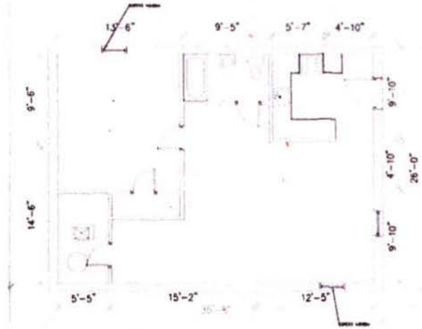
EXISTING BASEMENT FLOOR PLAN
