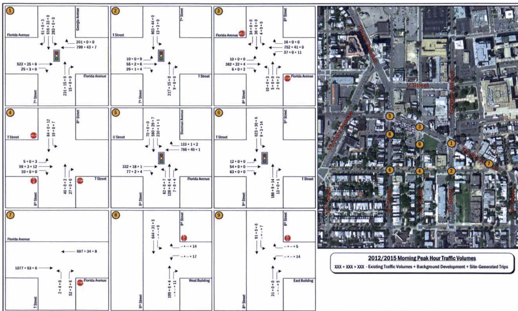
Figure 12: Morning Peak Hour Traffic Volumes
