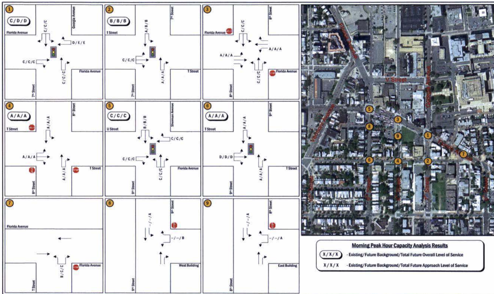
Figure 16: Morning Peak Hour Level of Service Results
