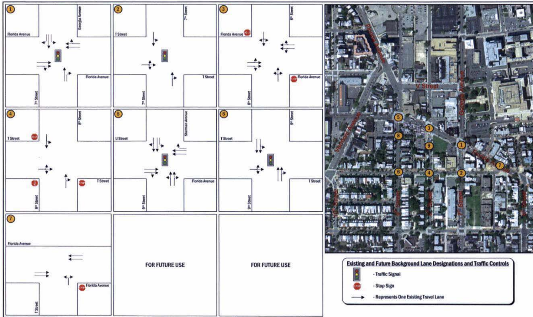
Figure 14: 2012 Existing and 2015 Background Lane Configurations
