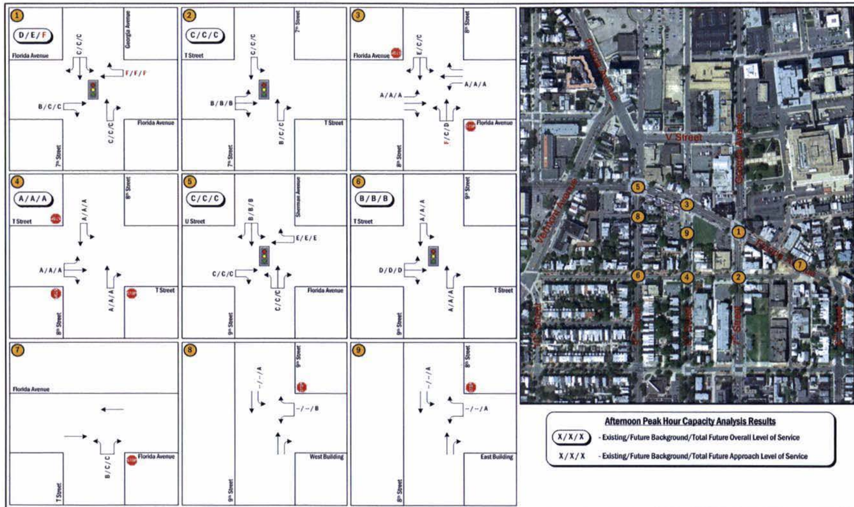
Figure 17: Afternoon Peak Hour Level of Service Results
