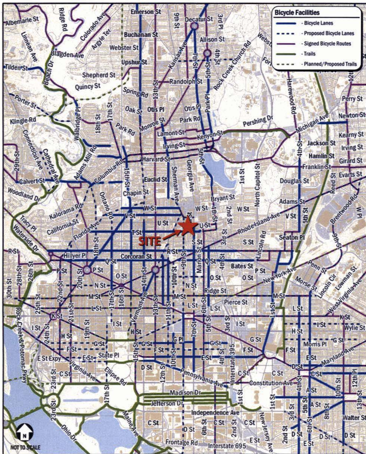
Figure 6: Existing Bicycle Facilities
