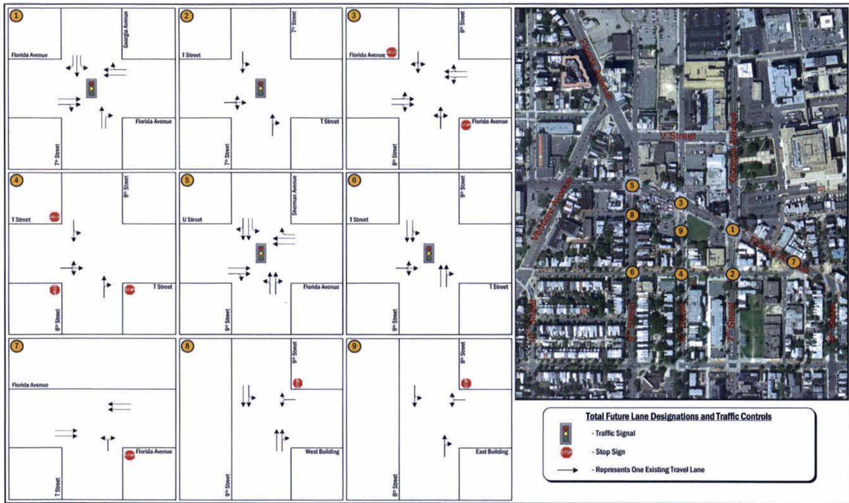
Figure 15: 2015 Future Lane Configurations
