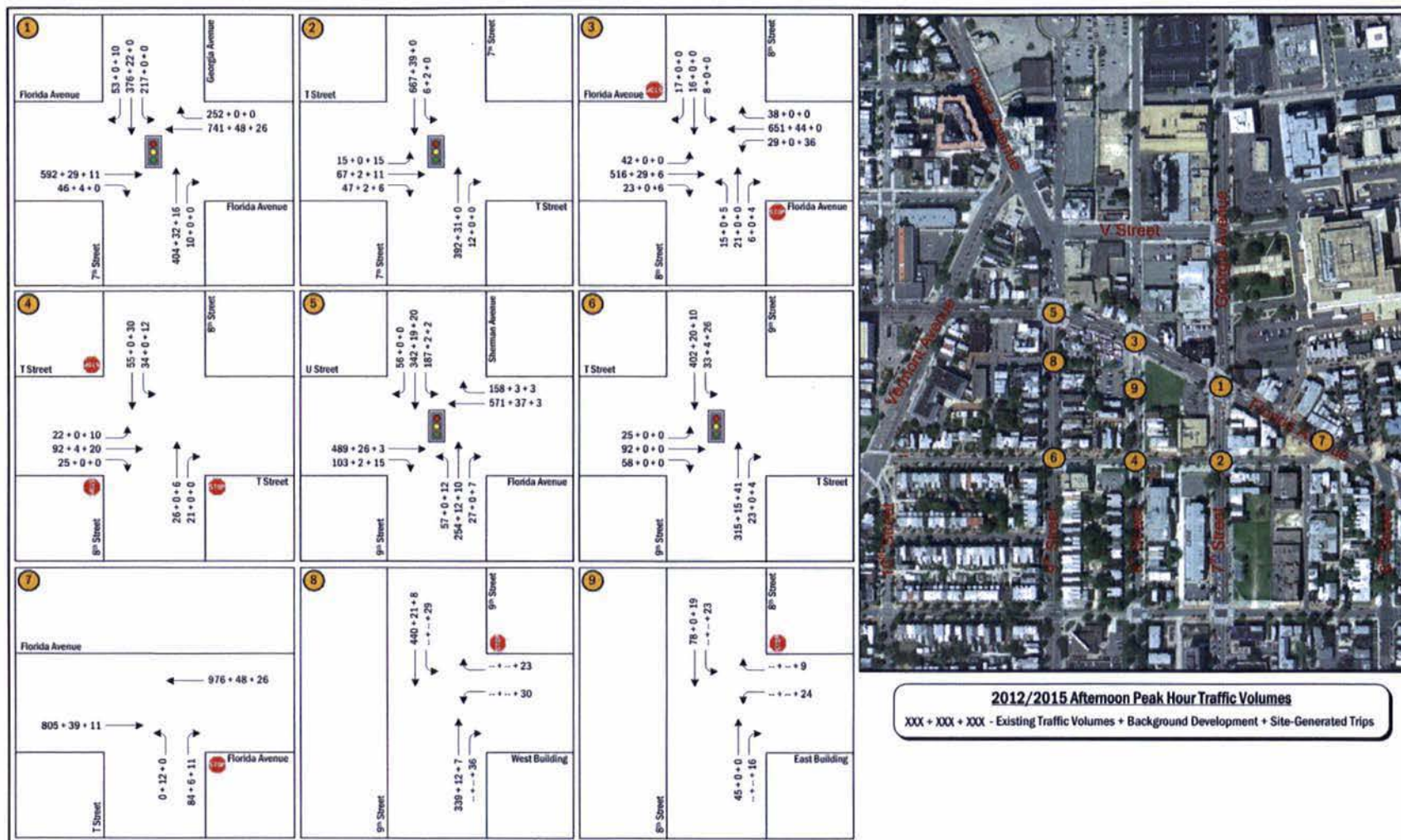
Figure 13: Afternoon Peak Hour Traffic Volumes
